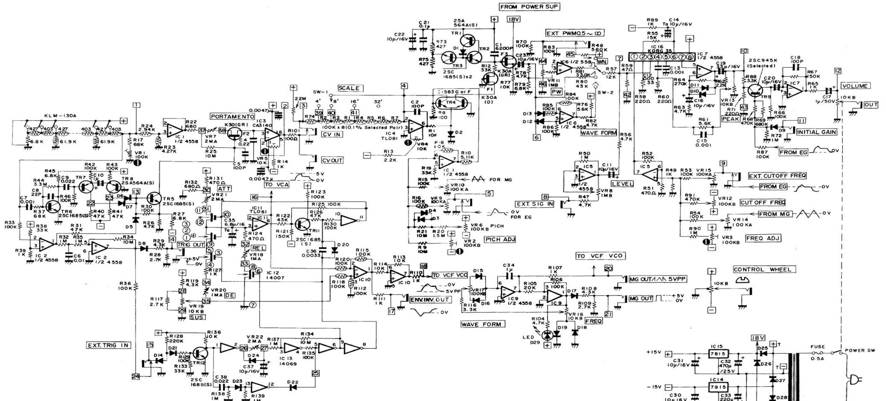
NOISE CIRCUIT NO.1 ( SERIAL NO.130000 ~ 132827 )
