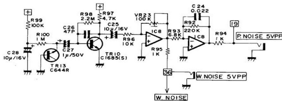
NOISE CIRCUIT NO.2 ( SERIAL NO.132828 ~ )
