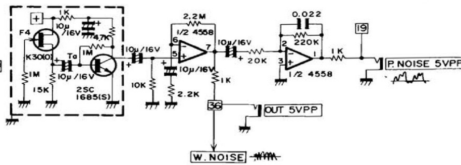
NOISE CIRCUIT NO.1 ( SERIAL NO.130000 ~ 132827 )
