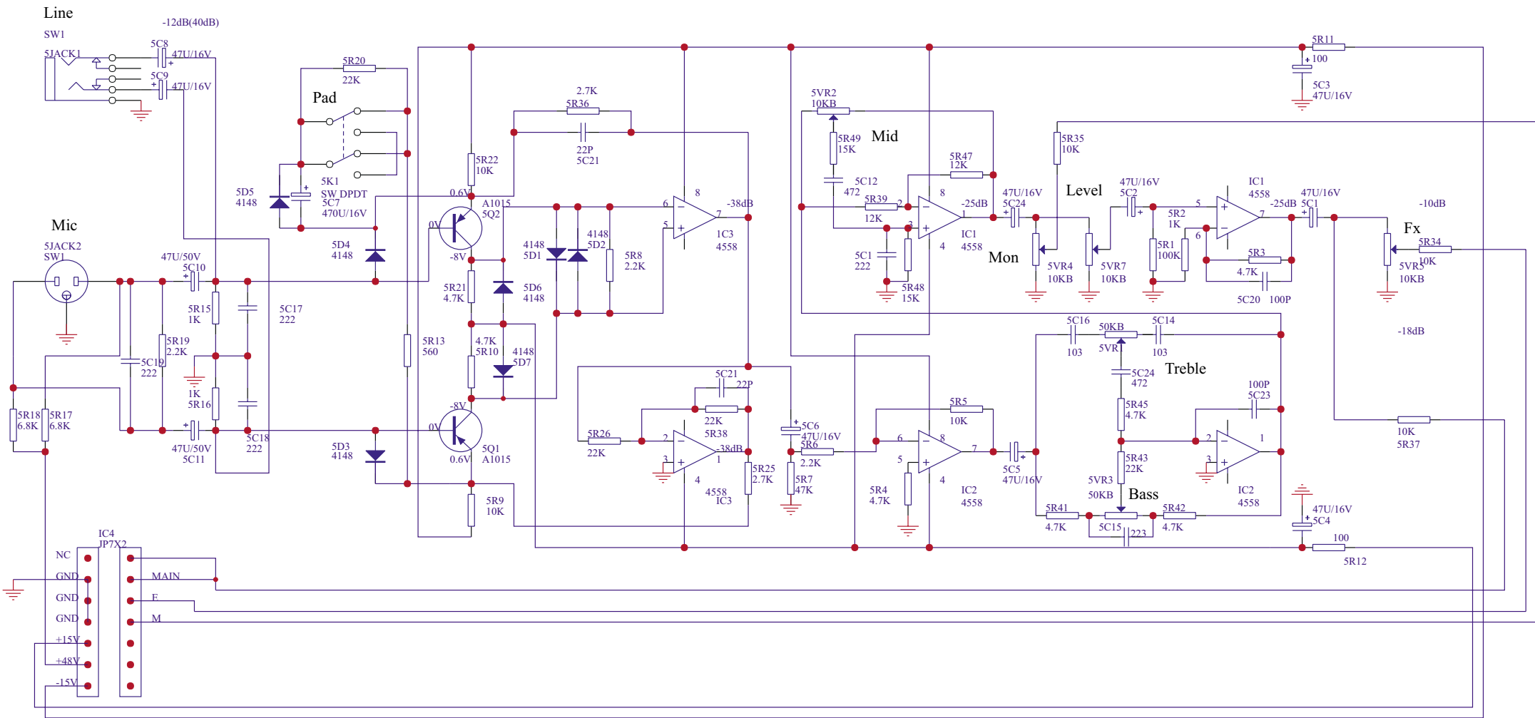
Laney CD640 Input Circuit 12/05/2003 SK.A97.148
