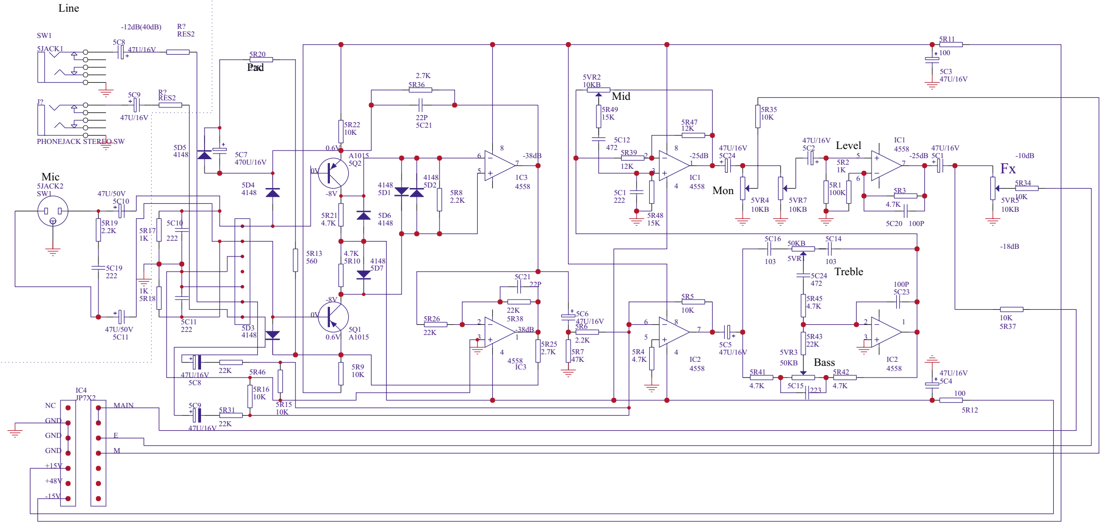
Laney CD640 Dual Mono Input Circuit 12/05/2003 SK.8.A97.150 SK.8.A97.154
