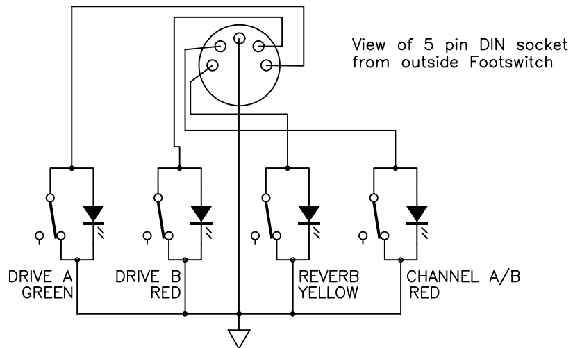
FS4 FOOTSWITCH
