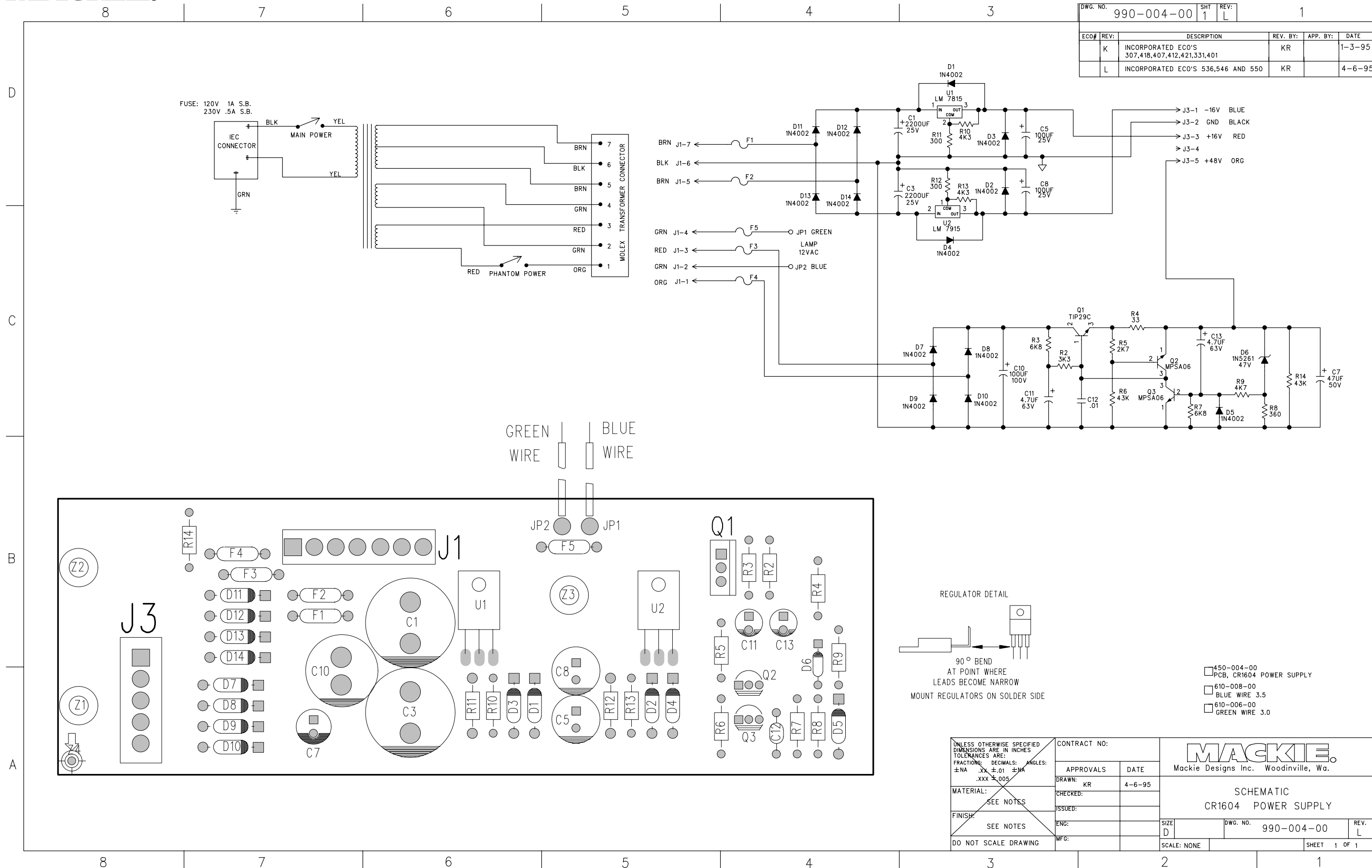
4-1 POWER SUPPLY 04 Rev L
