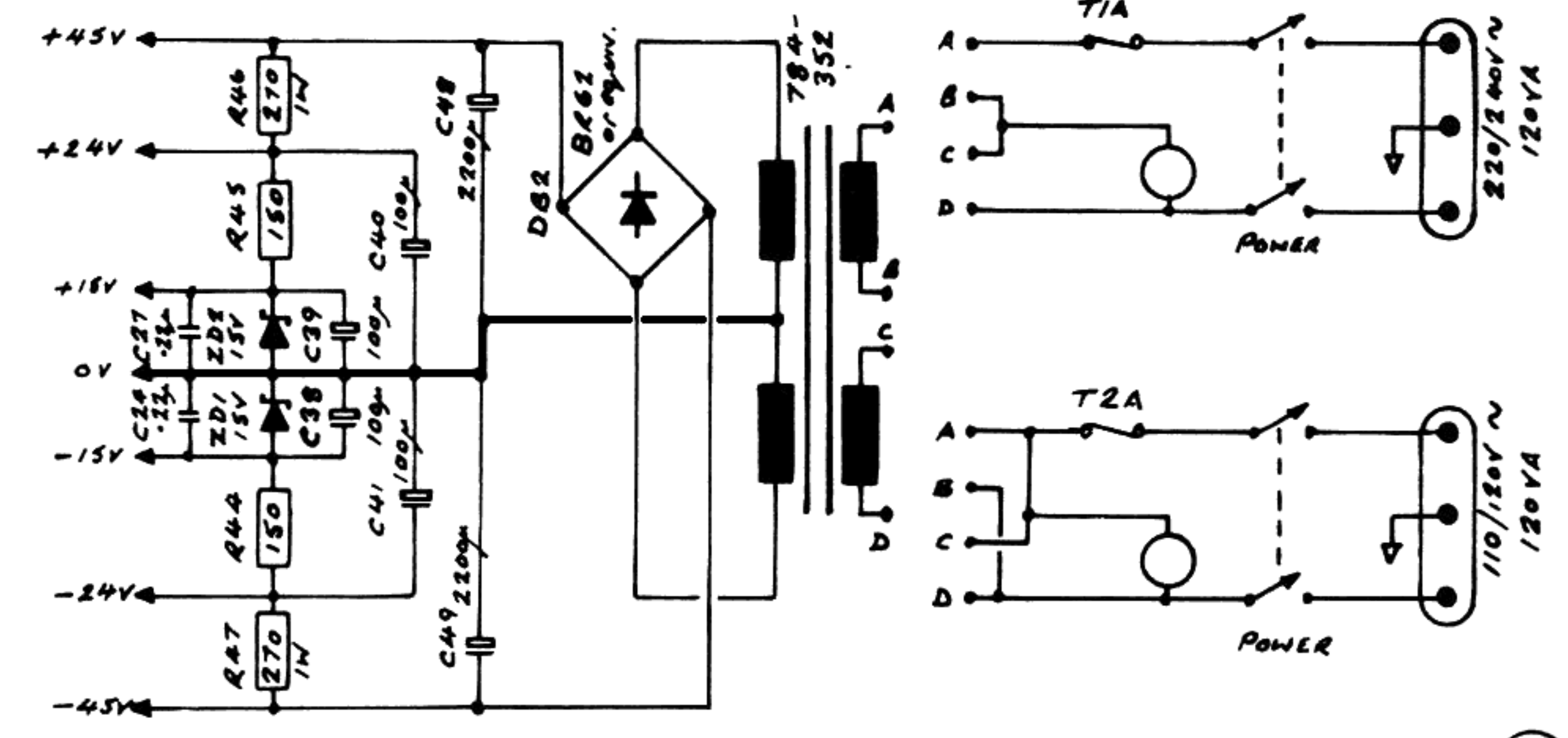
MARSHALL MODEL 5275 75 WATT 1x12 COMBO CIRCUIT DIAGRAM 1SS / 17-2-1984 S.C.
