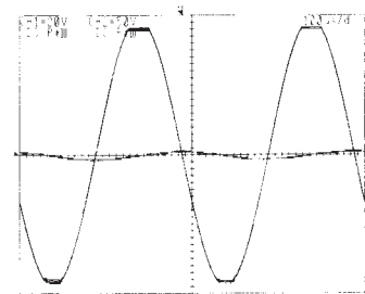
Even Clipping
