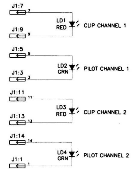
CX4/4T DISPLAY PCB SH-000048-00 2
