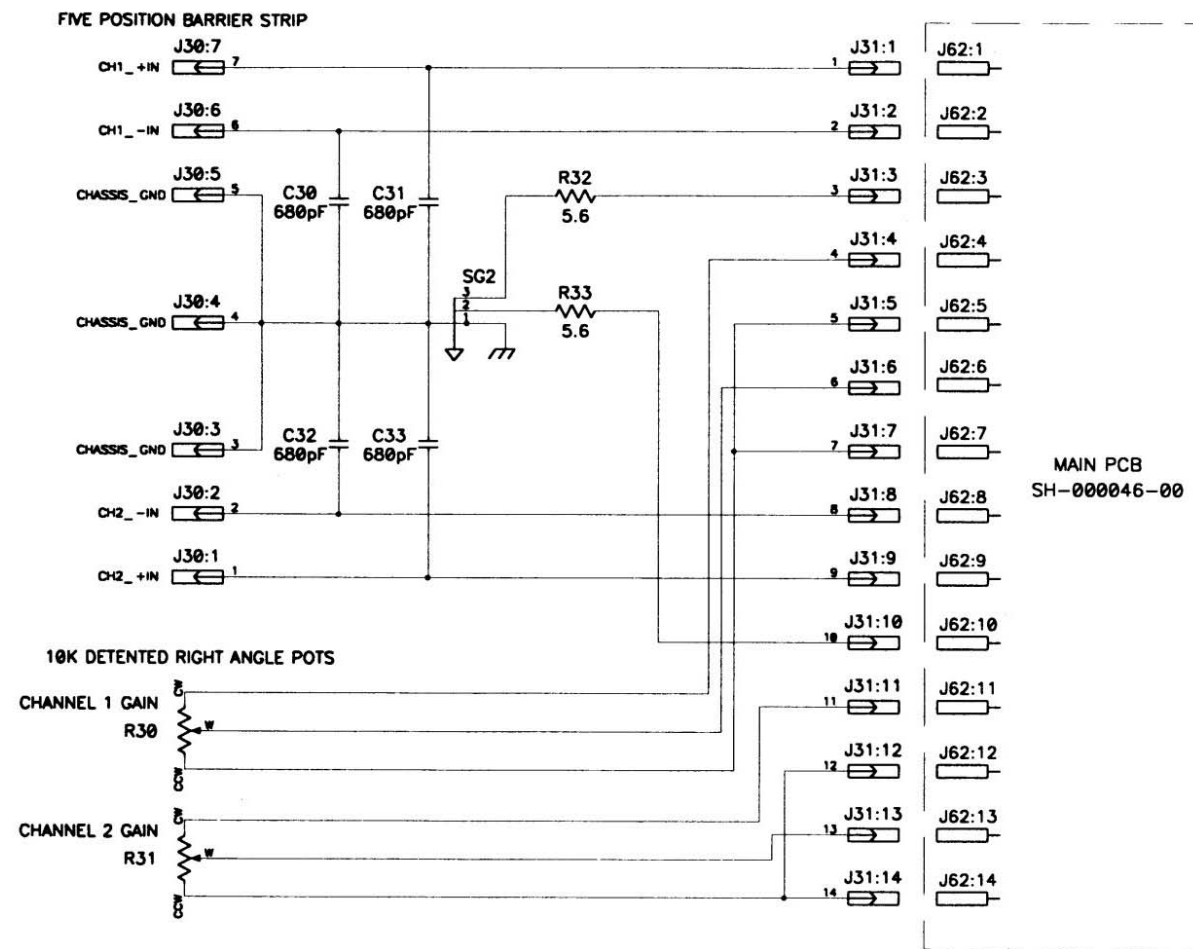
1. ALL RESISTOR VALUES ARE IN OHM 5%, 1/4W, CX4/4T INPUT PCB SH-000047-00
