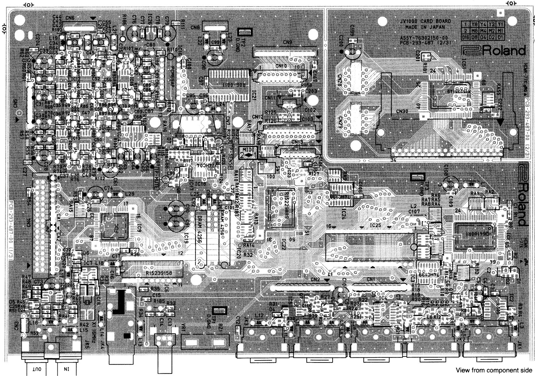
E MAIN BOARD-A ASS'Y ASSY 7630217000 (pcb 22935487)
