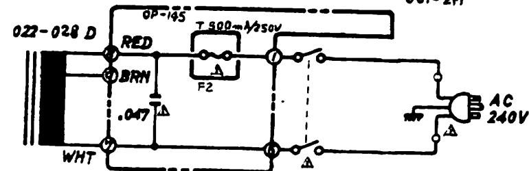
POWER SW. SDG-SP-302 001-217
