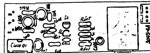
MIC LEVEL VR10 EVH6PA361C14 (026-141) MIC INPUT J4 HLJ0190-01-030 (009-046)
