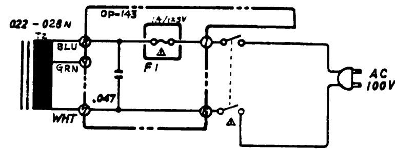
POWER SW. SDG-SP-001-1 001-215
