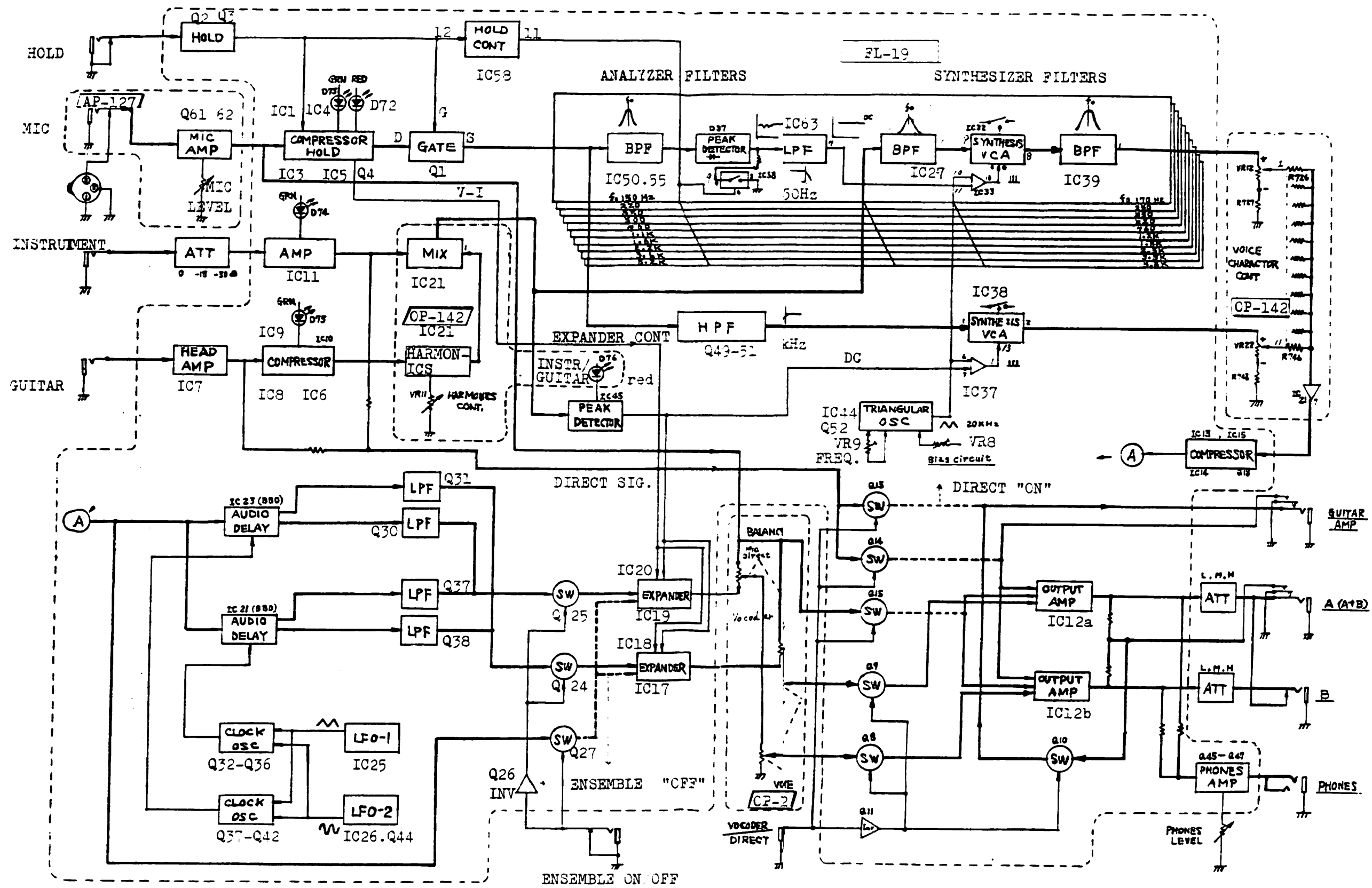
SVC-350 BLOCK DIAGRAM
