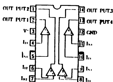
Connection Diagram (Top View)
