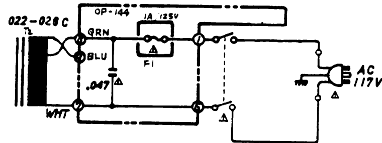
POWER SW. SDG-SP-001-2 001-216
