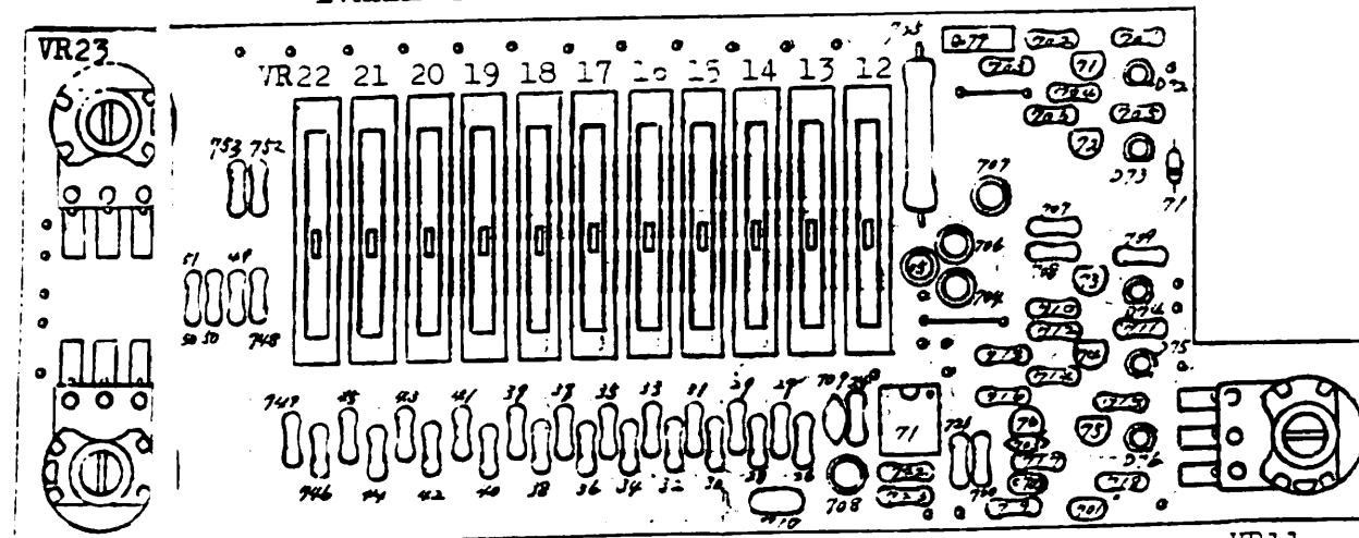
VOLUME! EWJ-EJA320B14 (026-155) HARMONICS EVH-EQA361 B14 (026-158)
