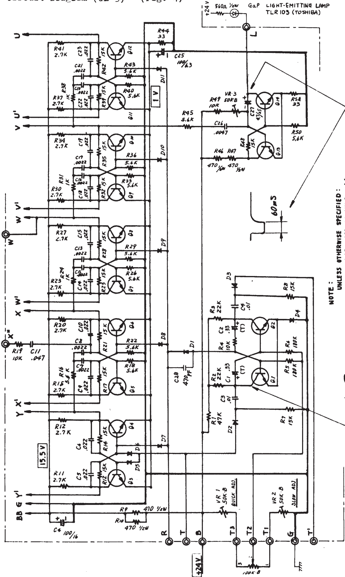
B. Circuit Diagram (GL-3) (Fig. 4)
