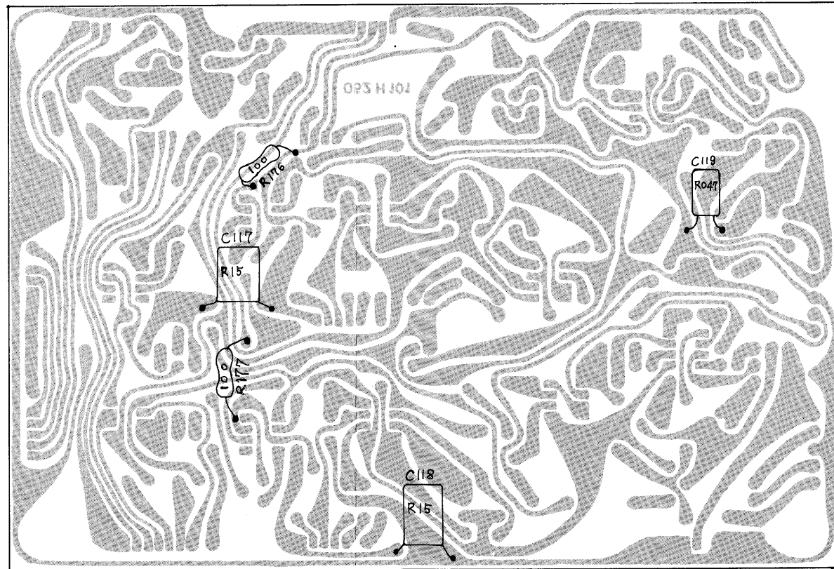
CVH-1 - PARTS ON THE FOIL SIDE
