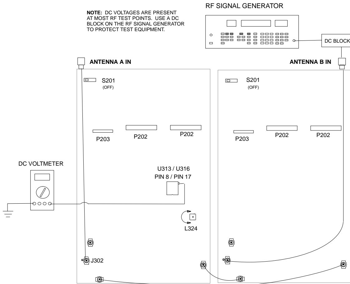
Figure 12. Channel B Second Mixer Coil Adjustment Connections
