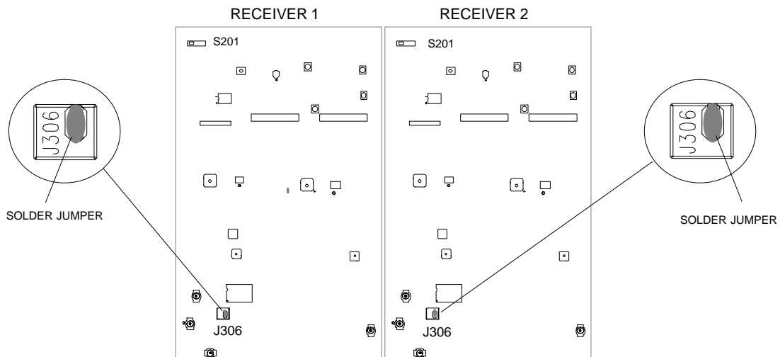
Figure 4. U4D Receiver Solder Jumper Locations
