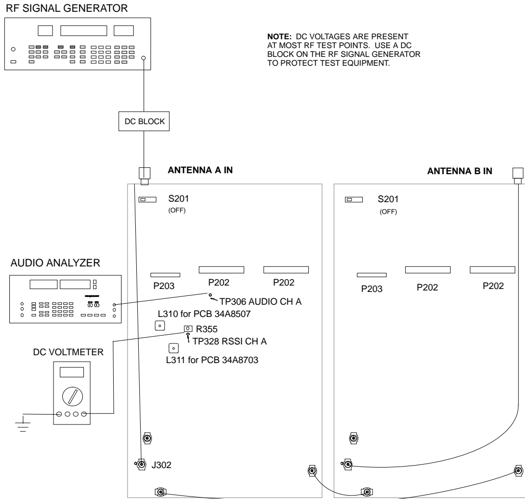
Figure 9. Channel A RSSI Alignment
