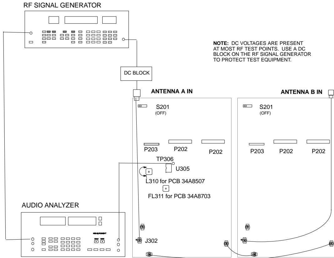
Figure 7. FM Detector Quadrature Coil Alignment Connections
