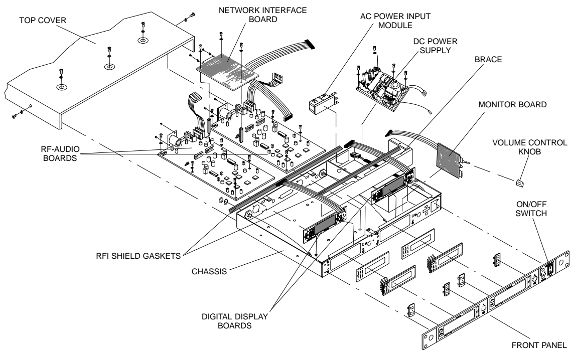
Figure 2. U4D Disassembly and Assembly
