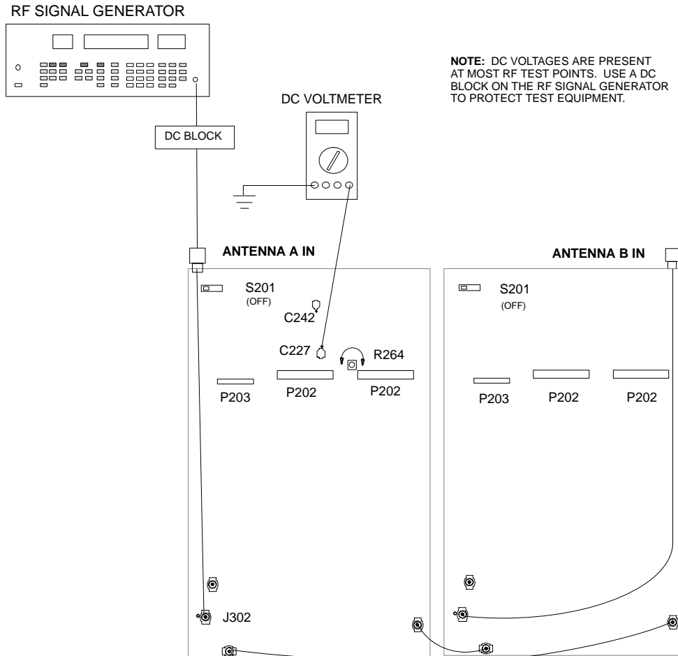
Figure 10. Channel A Noise Setup Connections
