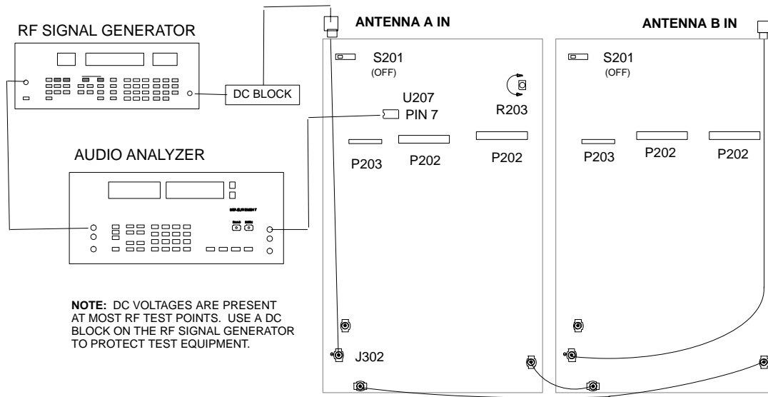
Figure 16. Channel A Audio Level Setup Connections
