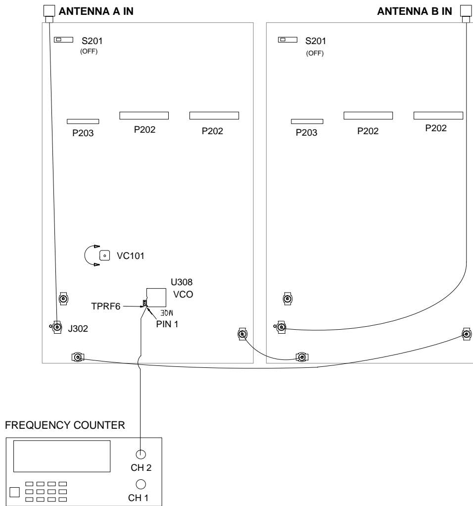
Figure 6. Local Oscillator Frequency Alignment
