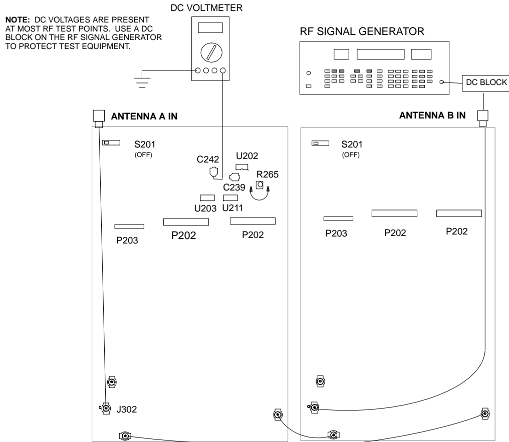
Figure 14. Channel B, Noise Setup Connections
