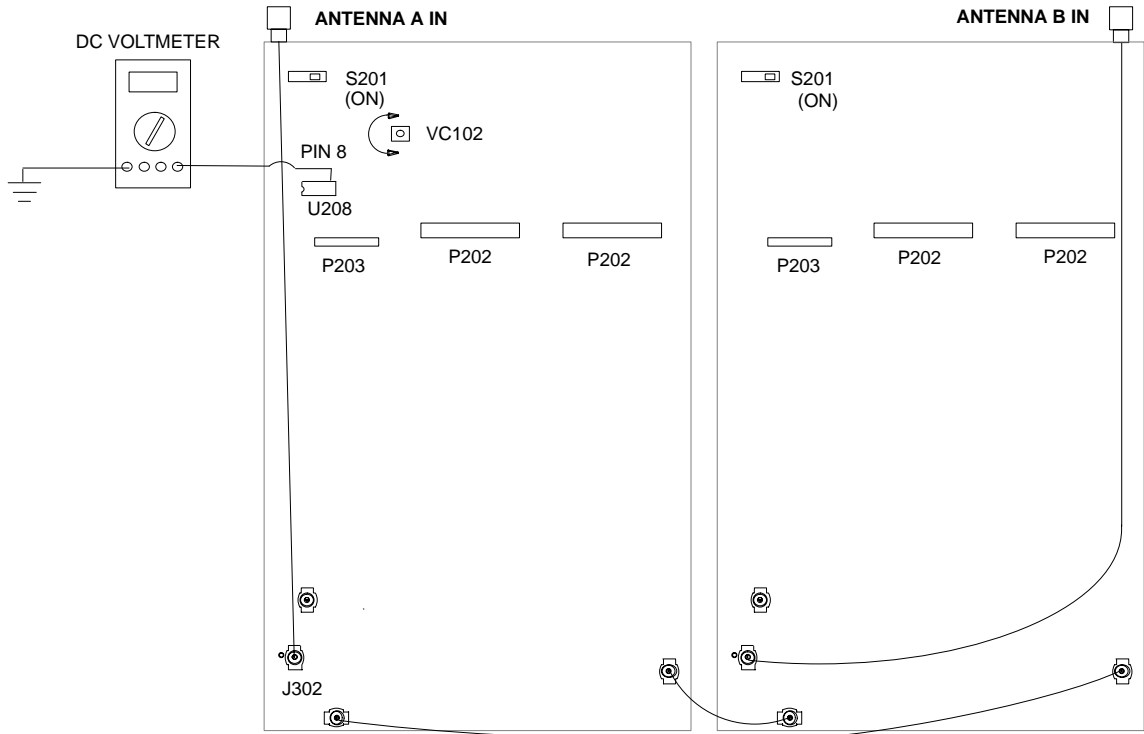
Figure 17. Tone Key Filter Alignment Connections
