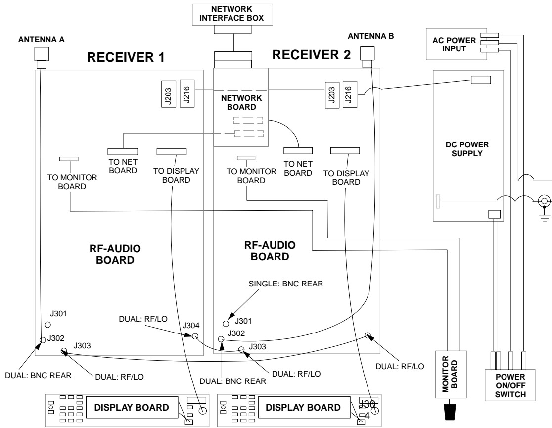
Figure 3. Final Cable Configuration
