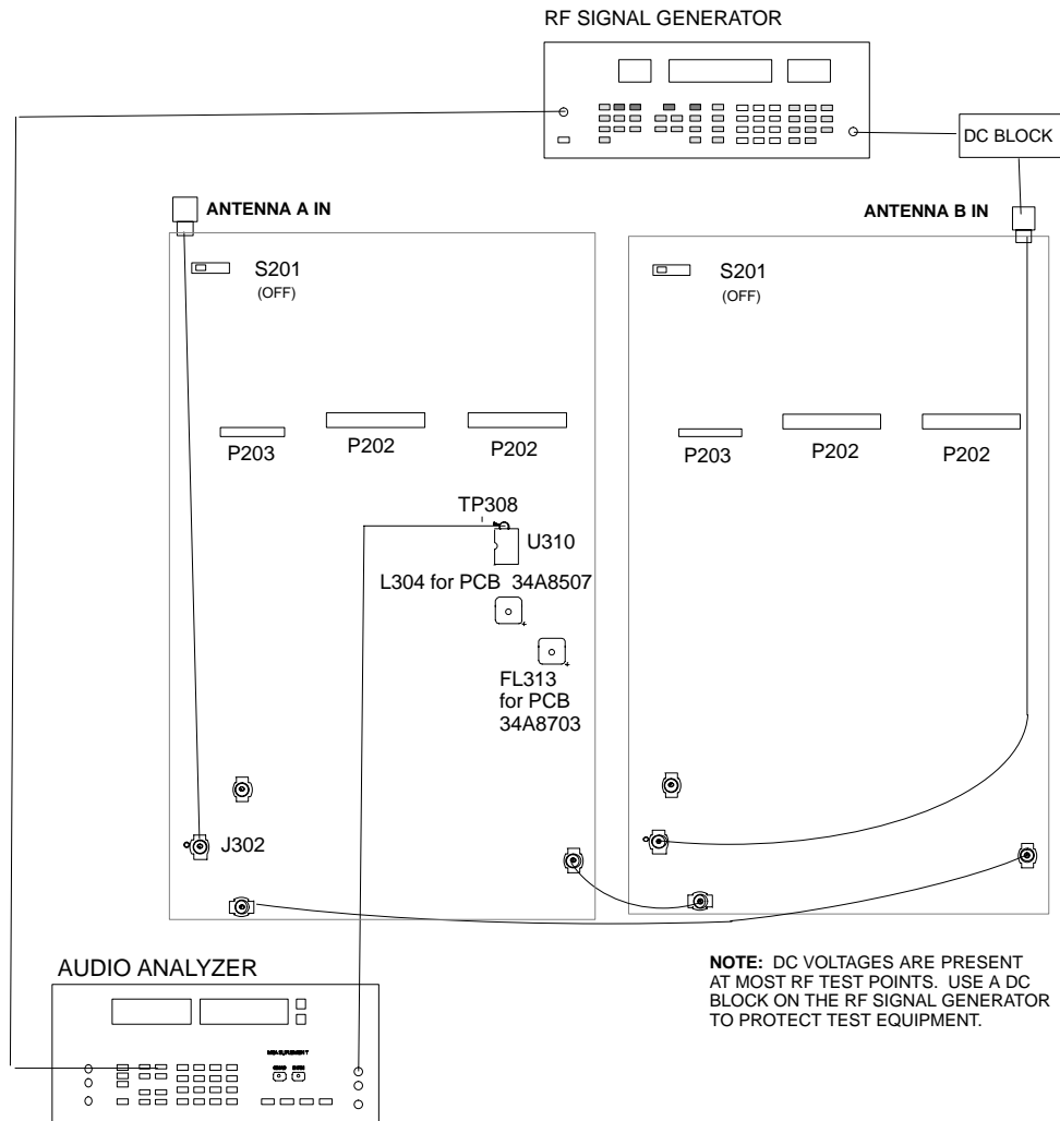
Figure 11. Channel B FM Detector Quadrature Coil Alignment
