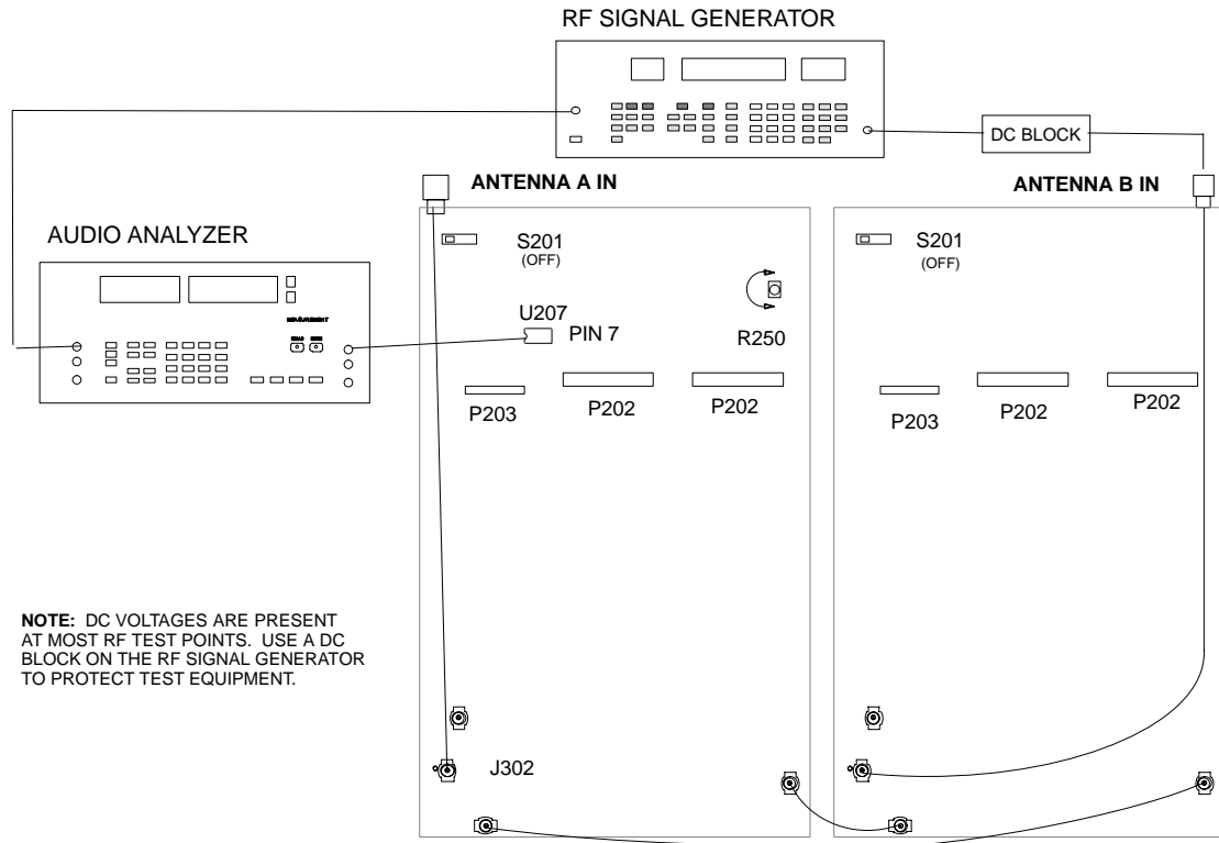
Figure 15. Channel B Audio Level Setup Connections
