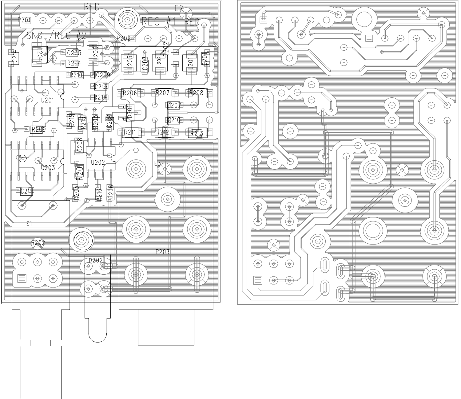
Figure 19. Headphone Monitor Printed Circuit Board Legend
