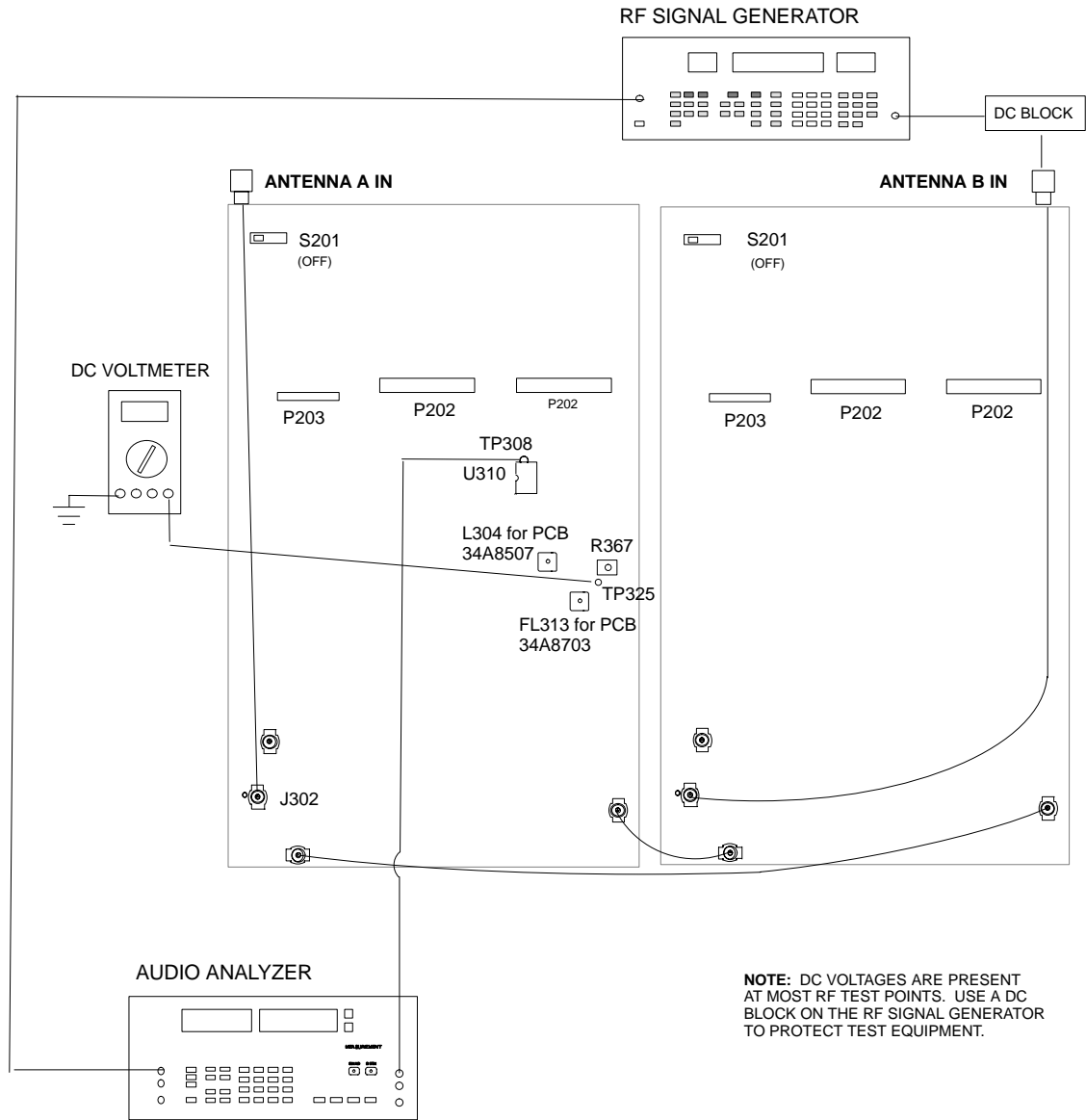
Figure 13. Channel B RSSI Alignment Connections
