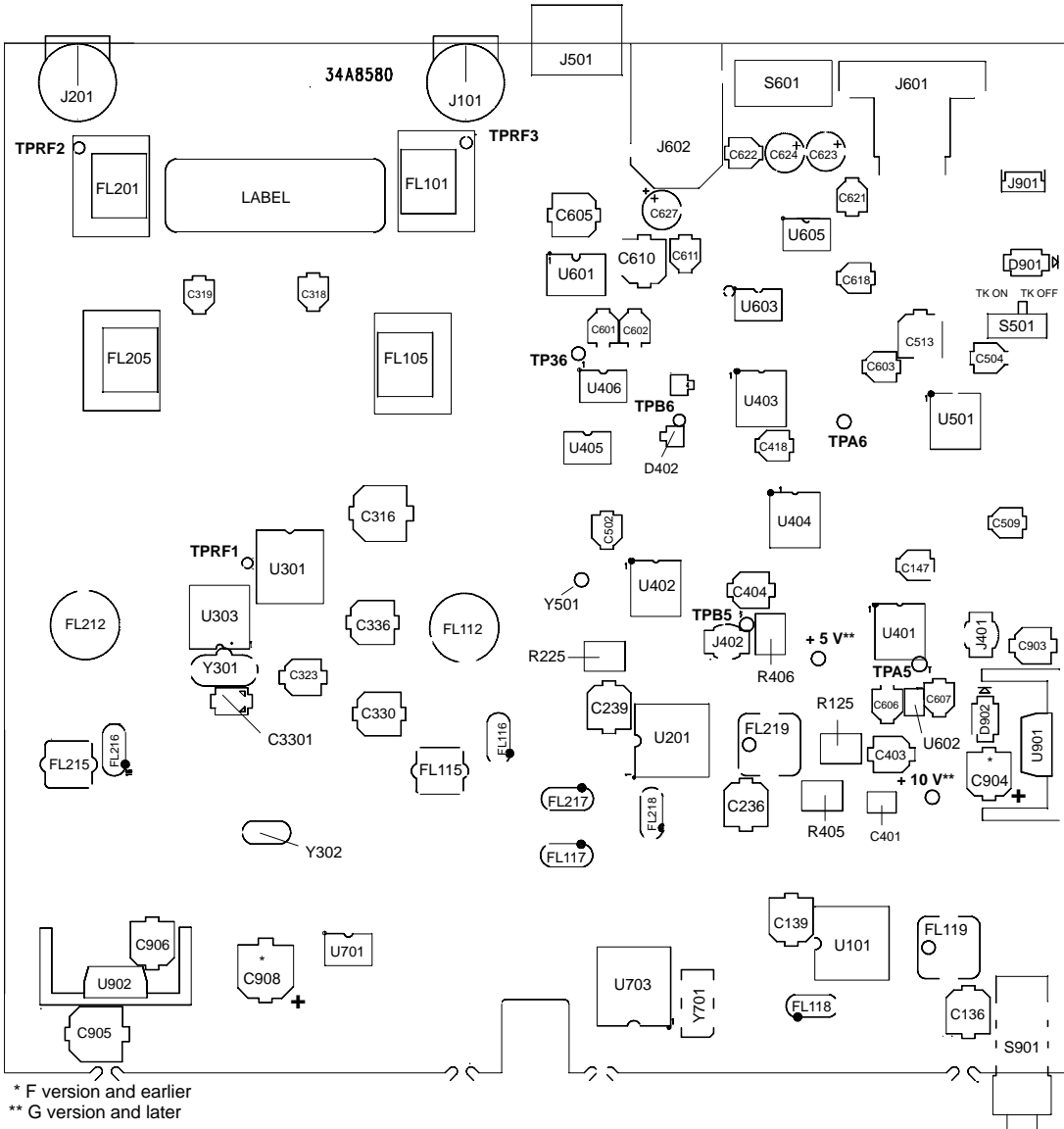
Figure 5. UC4 Major Test Component Locations
