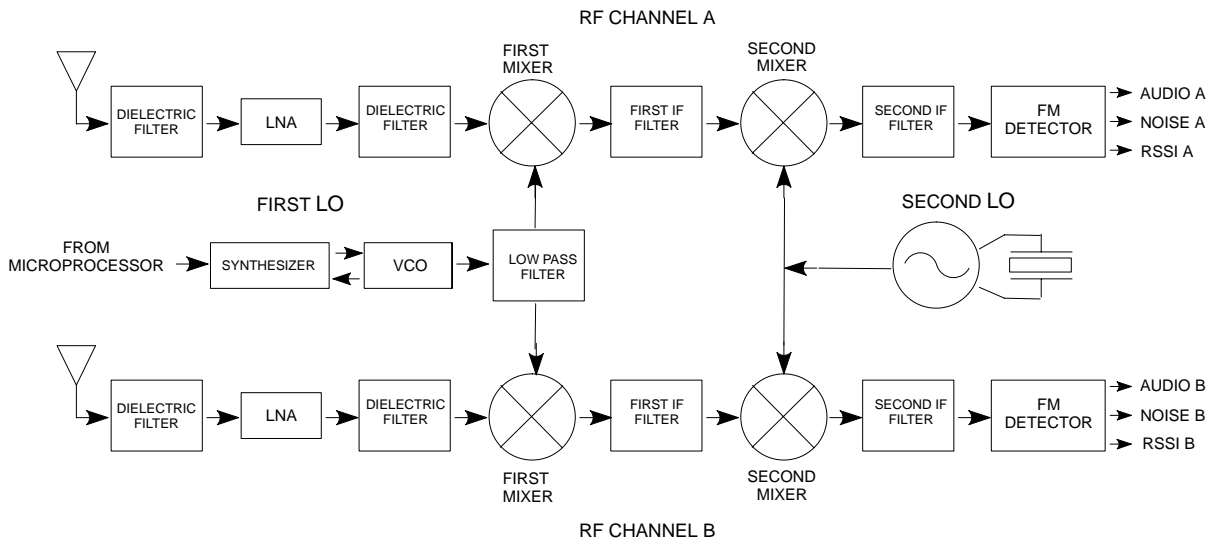
Figure 3. UC4 Rf Section Block Diagram
