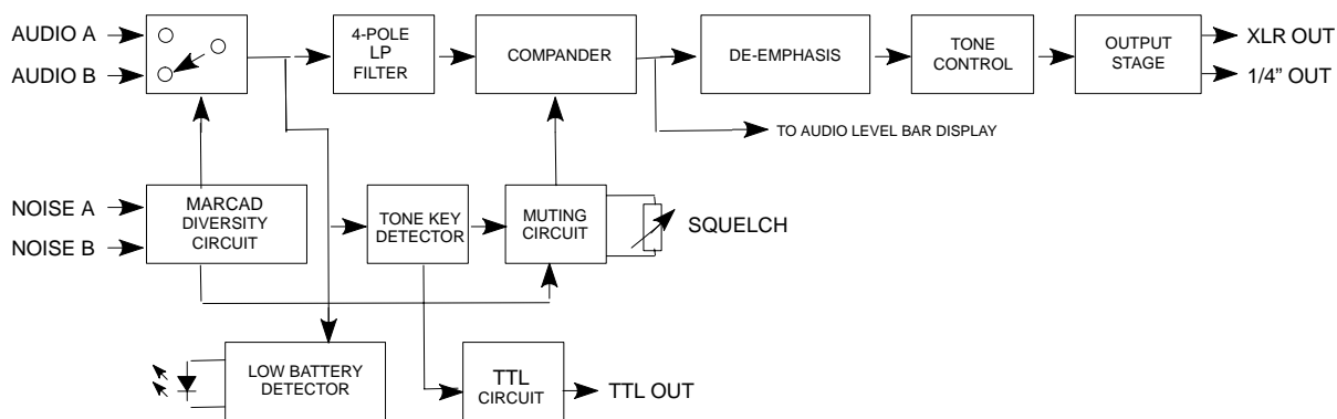
Figure 2. UC4 Audio Section Block Diagram
