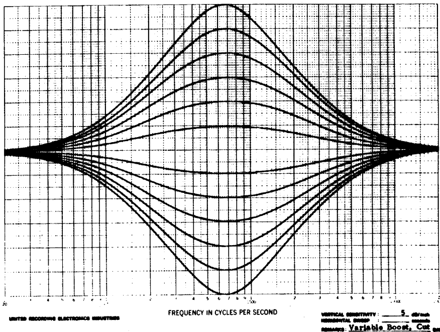
FIGURE 6-2. SINGLE PARAMETRIC FILTER SECTION ADJUSTED TO VARIOUS AMOUNTS OF BOOST OR CUT, WHILE THE BANDWIDTH (Q) REMAINS AT A CONSTANT WIDE (2 OCTAVE) SETTING. VERTICAL SENSITIVITY = 5 dB/in.
