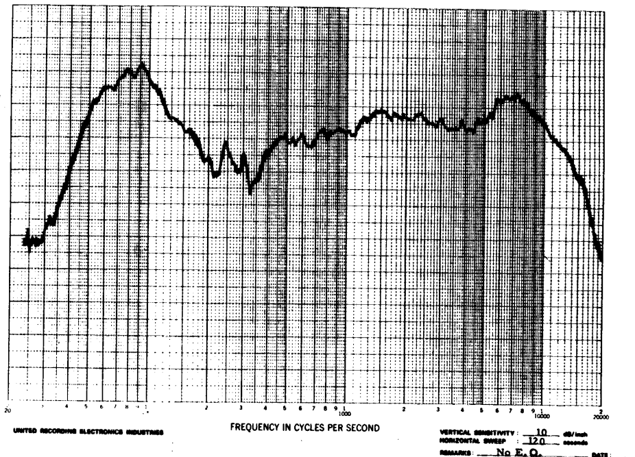
FIGURE 6-6. ACOUSTIC ANALYSIS OF A STUDIO MONITOR SPEAKER, MEASURED WITH A SWEEPED SINE WAVE WHICH WAS WARBLED WITH 1/3-OCTAVE BANDWIDTH. VERTICAL SENSITIVITY = 10 dB/in.
