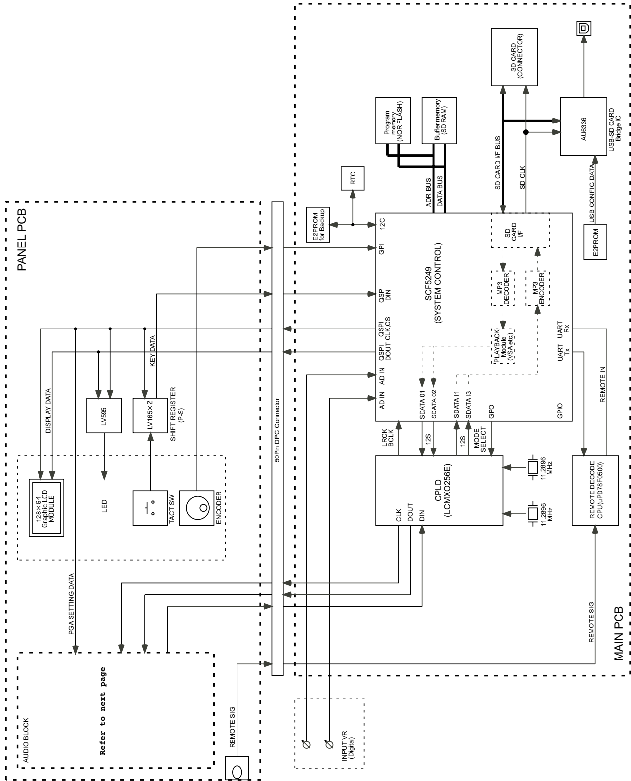
DR-100 H/W BLOCK DIAGRAM
