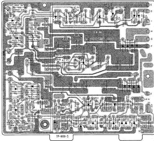
MIC JACK PCB ASSY
