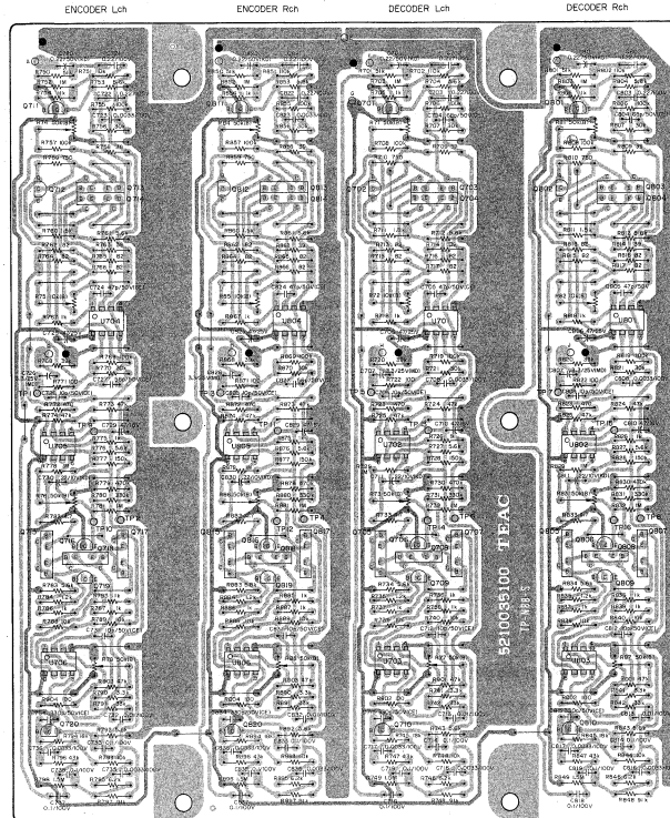
DBX PCB ASSY
