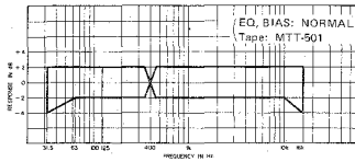
Fig. 5-8 Overall frequency response [NORMAL]
