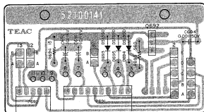
JOINT PCB ASSY
