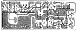
JOINT PCB ASSY
