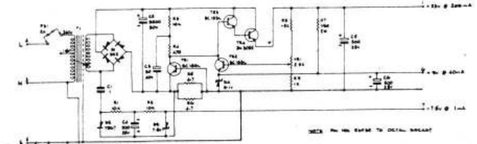
POWER SUPPLY UNIT P.C.B. 104 02
