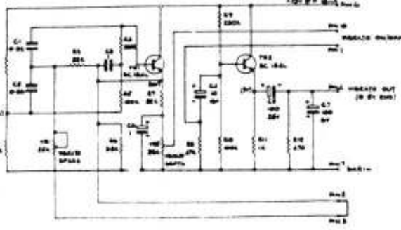
OPERATOR UNIT P.C.B. 104 02
