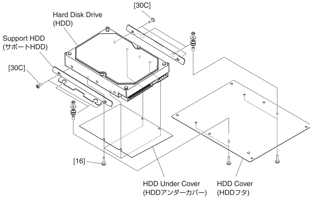
[16] Dish Head Screw UN#6x32-5 (WE878600) 小ネジ+ D I S H [30C] Dish Head Screw UN#6x32-5 (WE878600) 小ネジ+ D I S H
