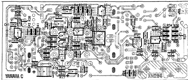
Pattern side
