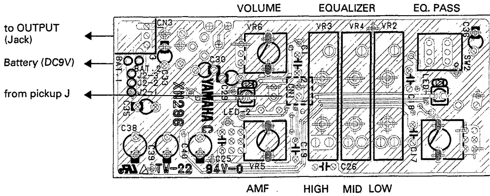
Components side
