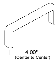
8571 U-SHAPE ALUMINUM OVAL BLACK HANDLE
