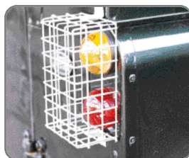
BR 1634 Single Galvanised Front Lampguard.
