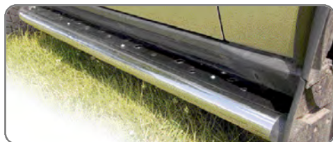
STC50032 Side Step for Disco 2.
