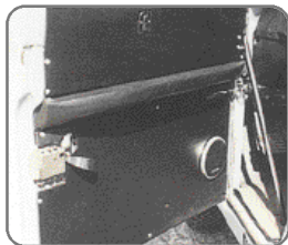
BA 049 Door Trim Kit for Series 2/3. Supplied as a kit to trim two front doors, available with armrest.
