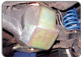
BA 125 Diff Guard for Discovery 1 & 2 (not LHD).
