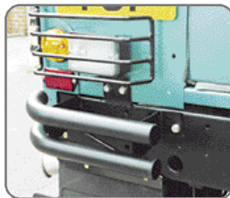
BA 090T Tubular bumperettes Black Nylon coated.
