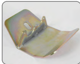
BA 3133 Diff Guard Slider Type - Rear.
