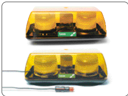
BA 4610 Xenon, 2 bolt fixing.
