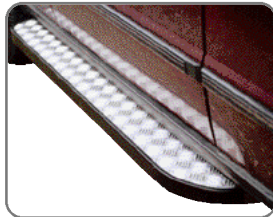
BA 092 Side Step with aluminium tread.
