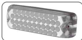
BA 4614 12V amber multi flash.
