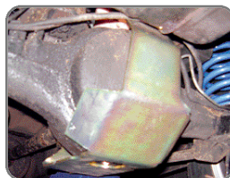
BA 125 Wrap around Diff Guard for Range Rover Classic. Front and Rear.
