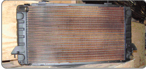
BR 3131H 4 row Radiator.
