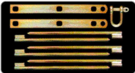
BA 2681 Ground Anchor Set.
