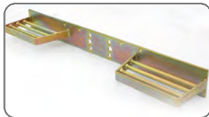
BA 172 Rear Step.
