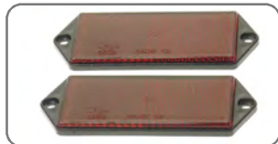
BA 3997 Red rectangular reflector (pack of two).
