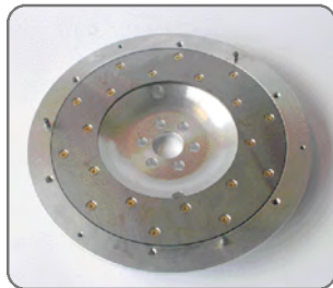
BA 2031 Flywheel to suit V8 engines.
