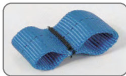
BA 2679 Rope Retainer.
