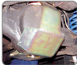
BA 125 Diff Guard for Defender NOTE: Not suitable for 110 rear 02MY on.
