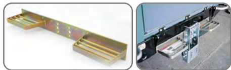
BA 172 Twin Rear Step.
