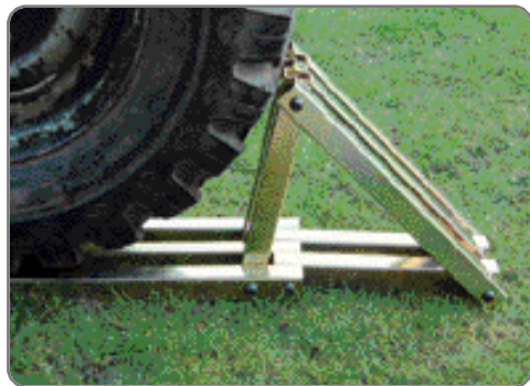
BA 5683 Towing Eye to suit Tubular Winch Bumpers.
