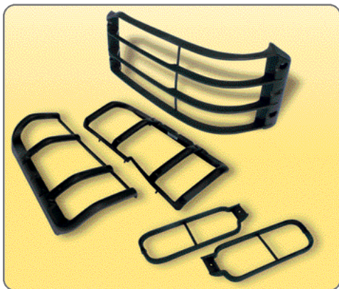
STC50026 Front Lamp Guards in plastic (Set of 2) – up to 03MY.
