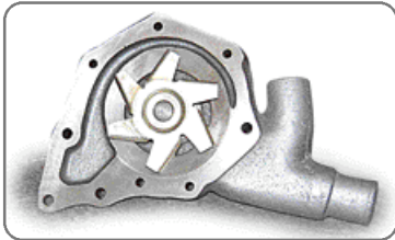
BWA 415 Heavy Duty Pump.
