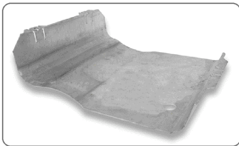
BA 3192 Fuel tank guard to suit Def 110 up to 1998.
