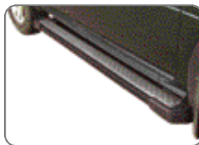
BFA 2032 Side Step Freelander 03-06.
