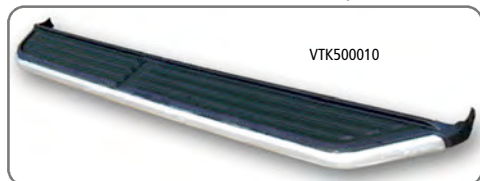
DGJ500010PMA Door Protection Strips.
