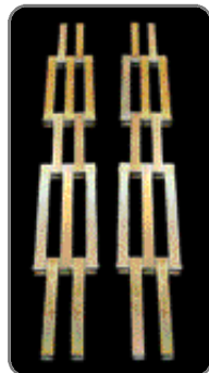
BA 2680 Winch Buddy.
