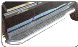
BA 100S Side Step in Stainless Steel (RR Classic).
