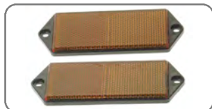
BA 3996 Amber rectangular reflector (pack of two).
