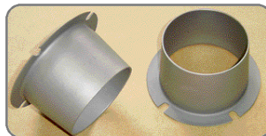
BA 3651 Rear pair of Dislocation Cones.
