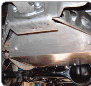
BA 3195G Fuel tank Guard to suit Defender 110 07> TD5 (Not with Tow Bar).
