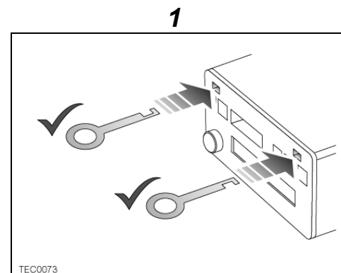
Correct fitment of radio removal keys illustrated
