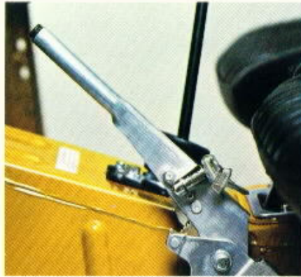
Parking brake with anti-theft locking device (LJ20)
