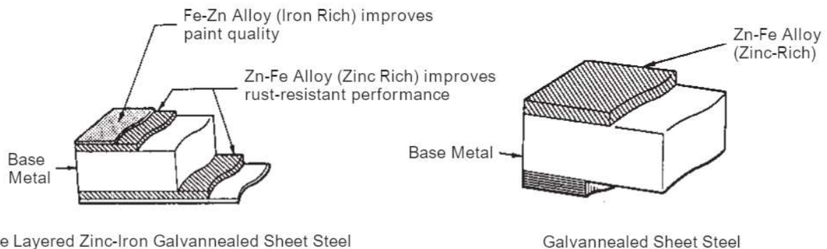
Double Layered Zinc-Iron Galvanized Sheet Steel
