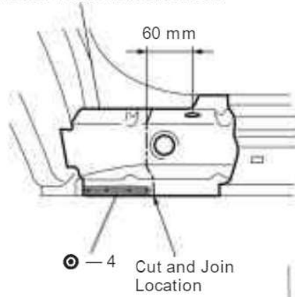
Rocker Panel Reinforcement
