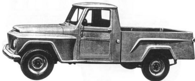
Fig. 5. PICK-UP JEEP modelos 9121 — 9221
