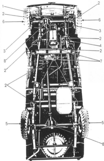
Chassi do Pick-Up Jeep 4 x 4 (9221)
