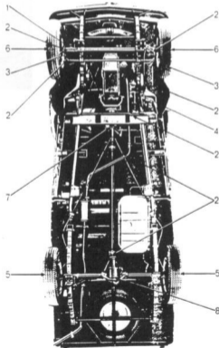
Chassi do Pick-Up Jeep 4 x 2 (9121 e 9122)
