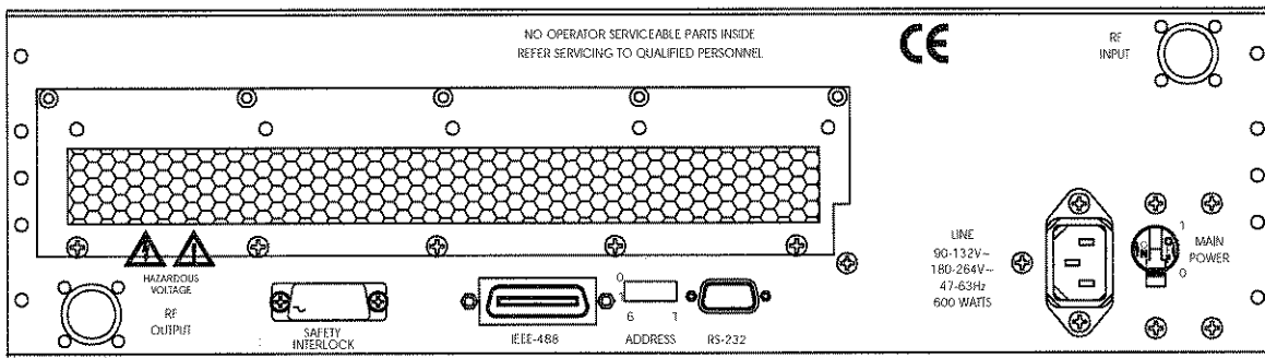
Figure 2-2 Model 10S1G4A Rear Panel
