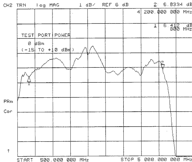
Figure 4.3.8.2 Typical Response: Input A6-Front Panel RF Output
