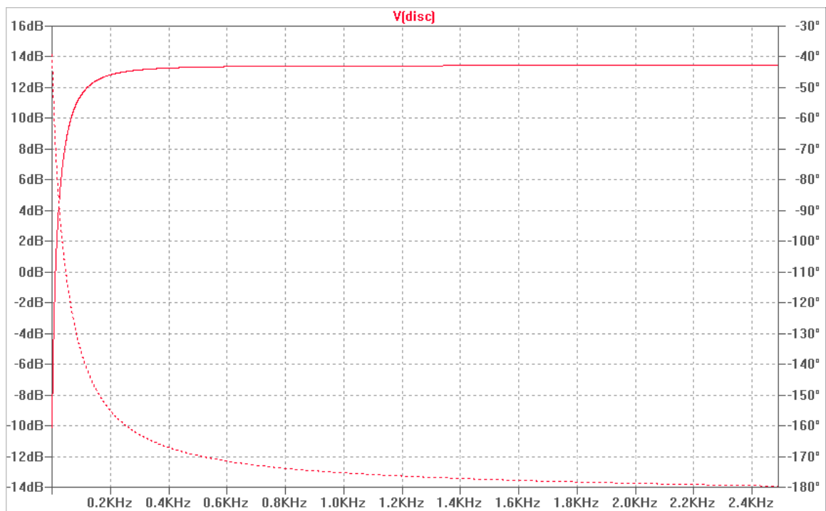
RX filter response, EQ jumper installed
