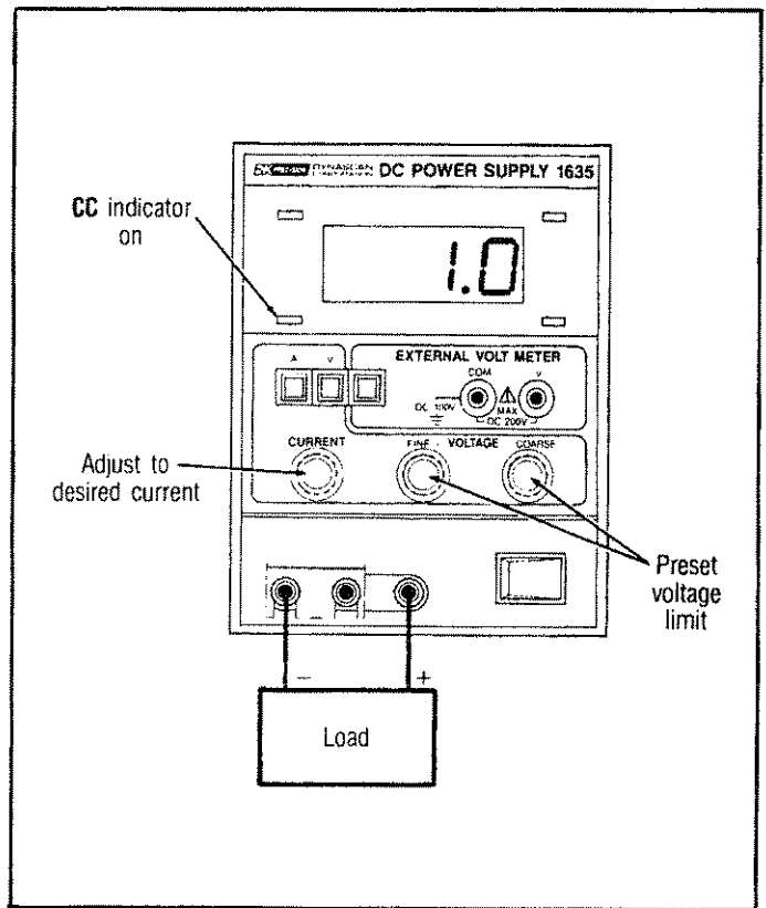
Fig. 6. Typical Constant Current Operation.
