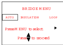
Figure 6 - Menu Bridge
