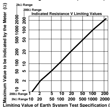
Limiting Value Curve (VDE 0413)
