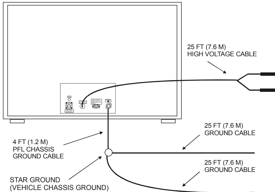
Figure 5-3 Ground System Diagram, Permanent Connections
