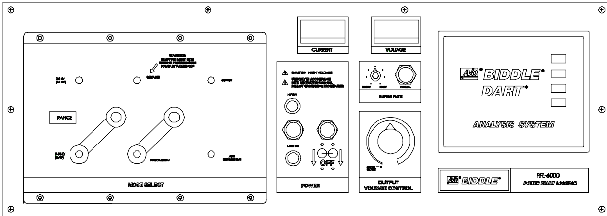
Figure 5-1 Controls
