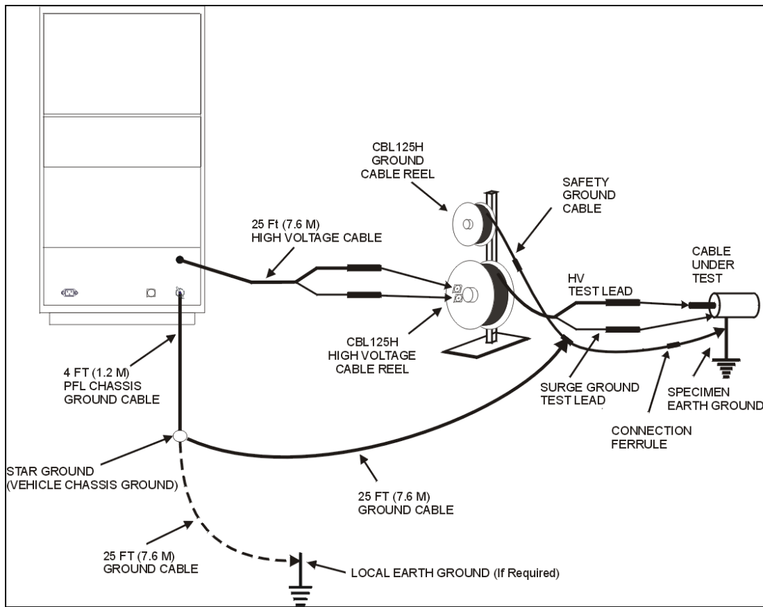
Figure 1: CBL125H Connections
