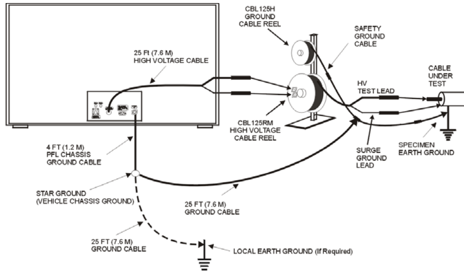
Figure 5-4 Temporary Connections
