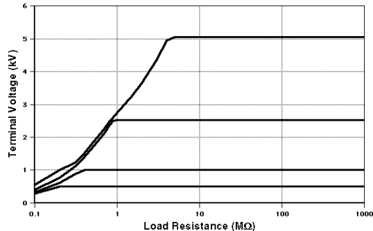
Typical Terminal Voltage Characteristics
