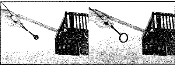
Figure 21. H and E field probes are being used to diagnose a problem on a printed circuit board. (By mapping the rate of roll-off of the H and E fields, the source impedance may be determined.)
