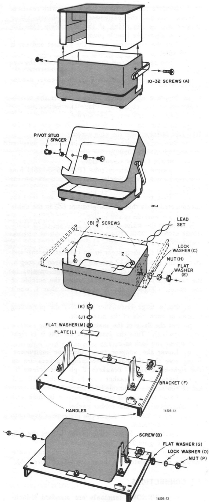
Figure 1-4. Rack mounting the 1650-B.
