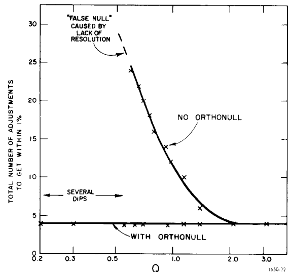
Figure 4 - 3. Number of balances vs Q.
