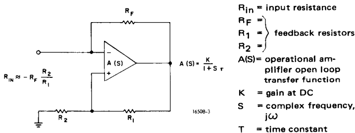
Figure 3-5. Operational amplifier.
