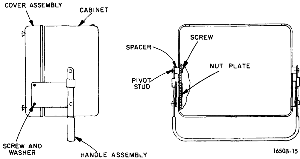
Figure 6 - 7. Complete cabinet assembly (P/N 4182-2002).
