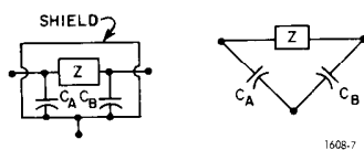
Figure 3-10. Shielded three-terminal impedance.
