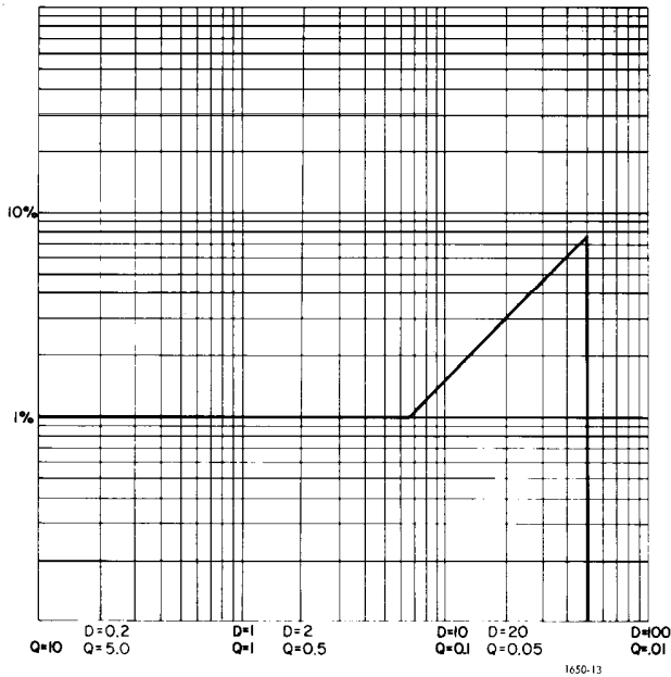
Figure 4-4. Accuracy vs D or Q.
