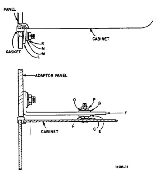
Figure 1-5. Detail view of panel mounting.
