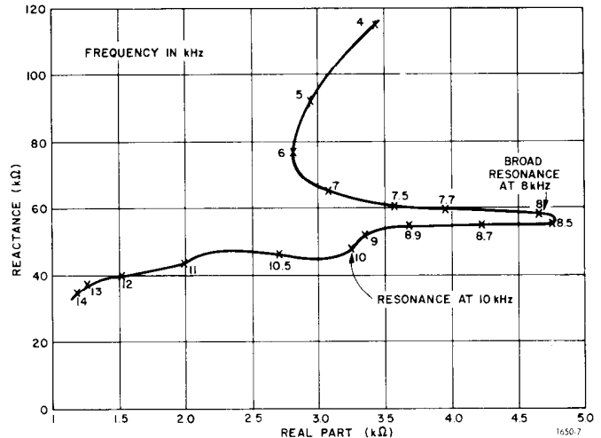
Figure 3-9. Typical impedance-vs-frequency response of a piezoelectric microphone.
