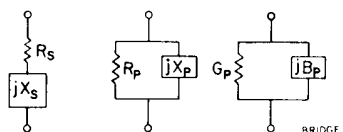
Figure 5-5. Series and parallel components of impedance.
