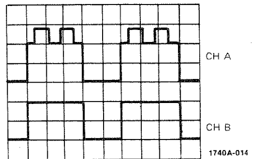
Figure 12a. Channel A With Desired Signal and Unwanted Components. Channel B With Only Unwanted Components.
