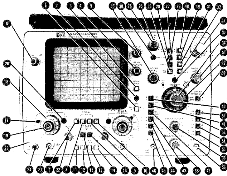
Figure 27. Front-panel Controls
