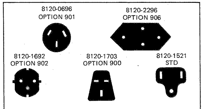
Figure 1. Power Receptacles
