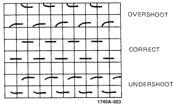
Figure 4. Probe Compensation
