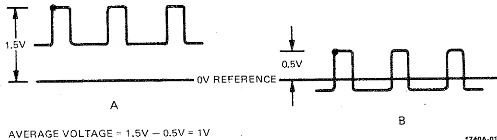
Figure 11. Average Voltage
