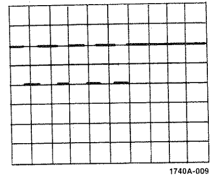
Figure 7b. Mixed Sweep Display
