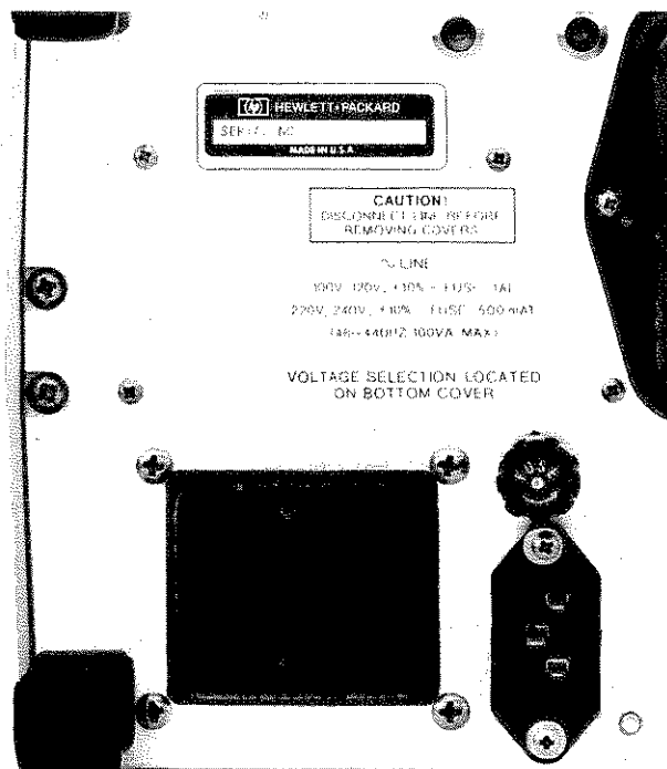
Figure 3. Fuse Replacement
