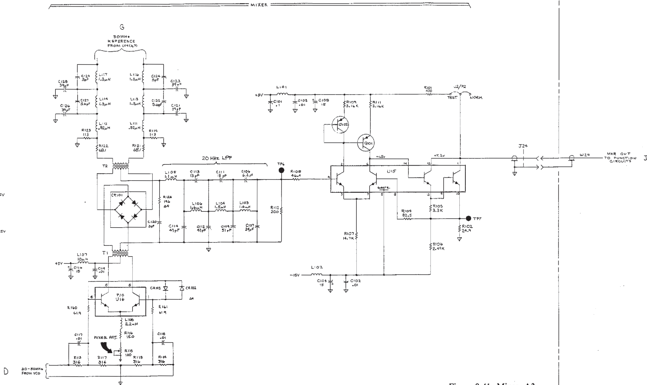
Figure 8-41. Mixer, A3. 8-H-3/8-H-4
