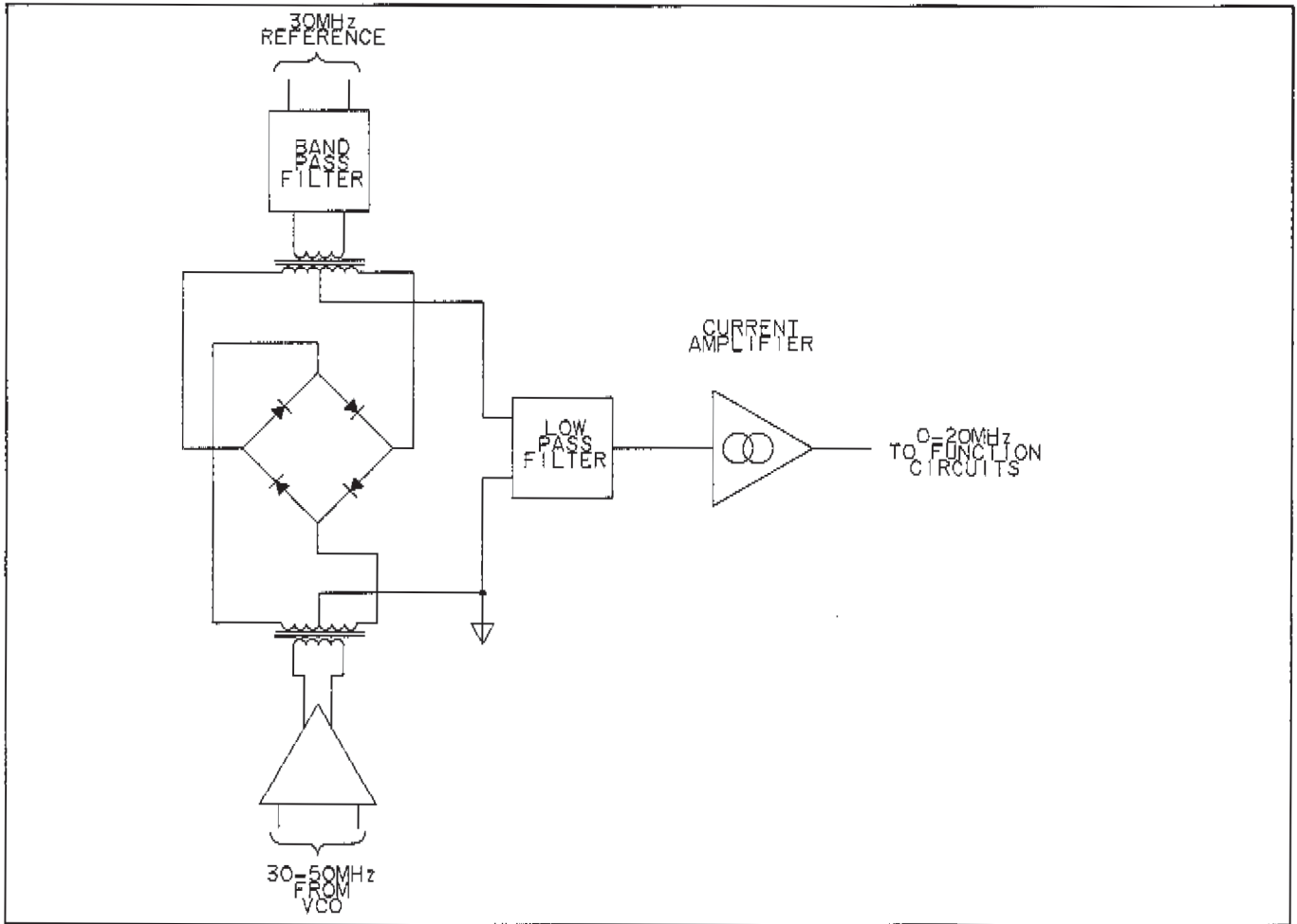
Figure 8-16. Mixer Diagram.
