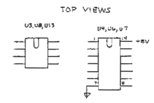
Figure 8-40. 30 MHz Reference and Dividers, A3. 8-G-3/8-G-4
