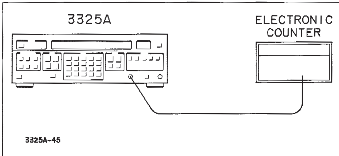
Figure 4-6. Frequency Accuracy.
