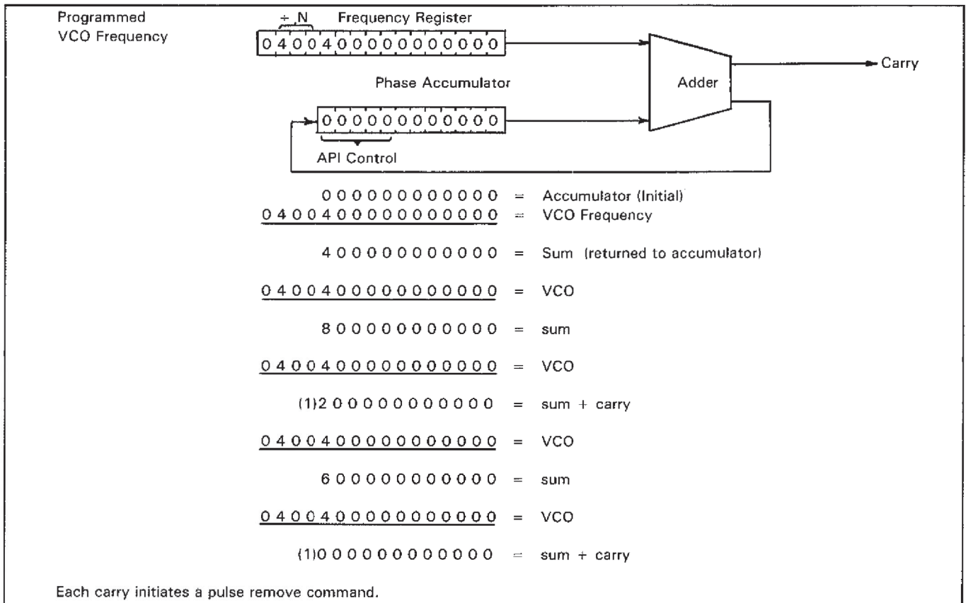
Figure 8-12. Phase Accumulation.
