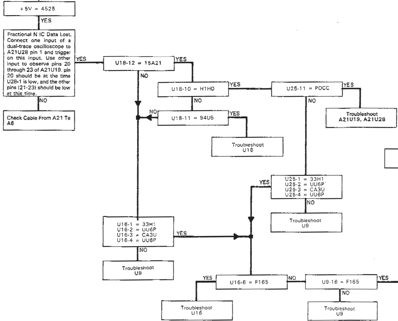
Figure 8-35(b). Signature Analysis Test 5. 8-C-33/8-C-34
