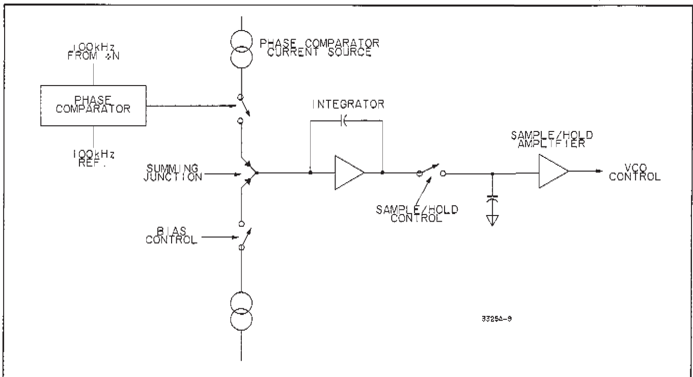
Figure 8-9. Phase Detector.
