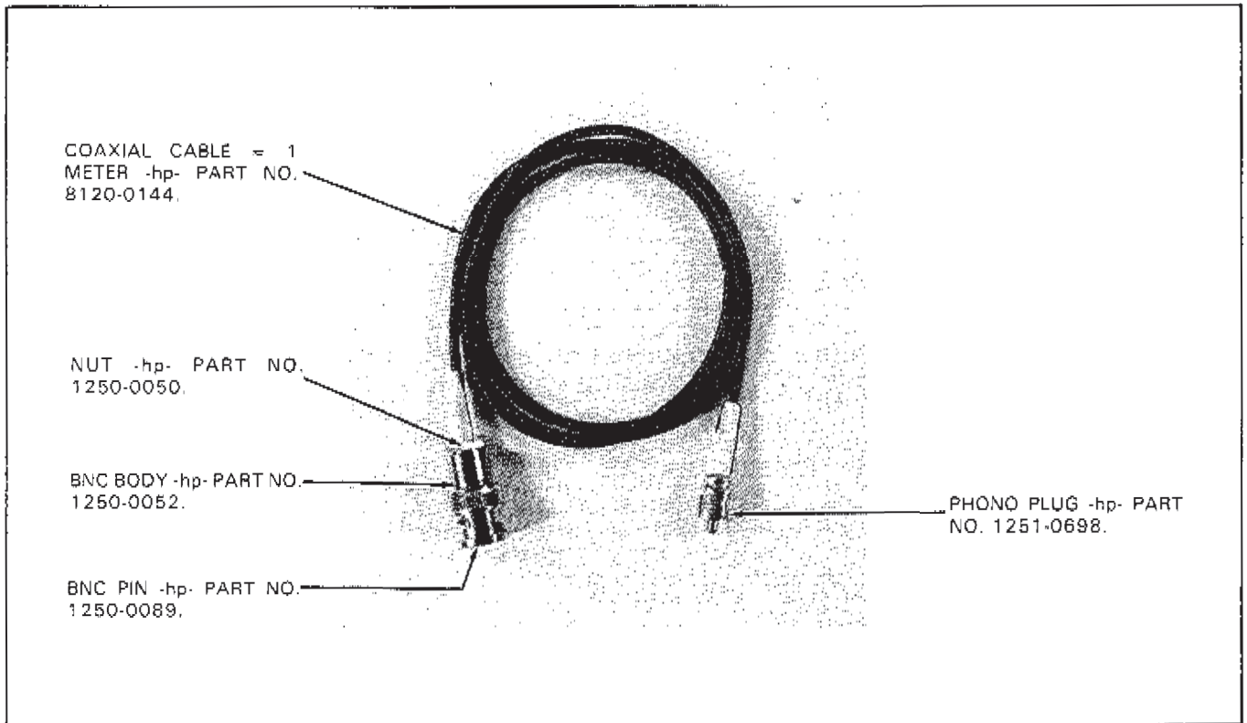
Figure 8-27. Adapter Cable.
