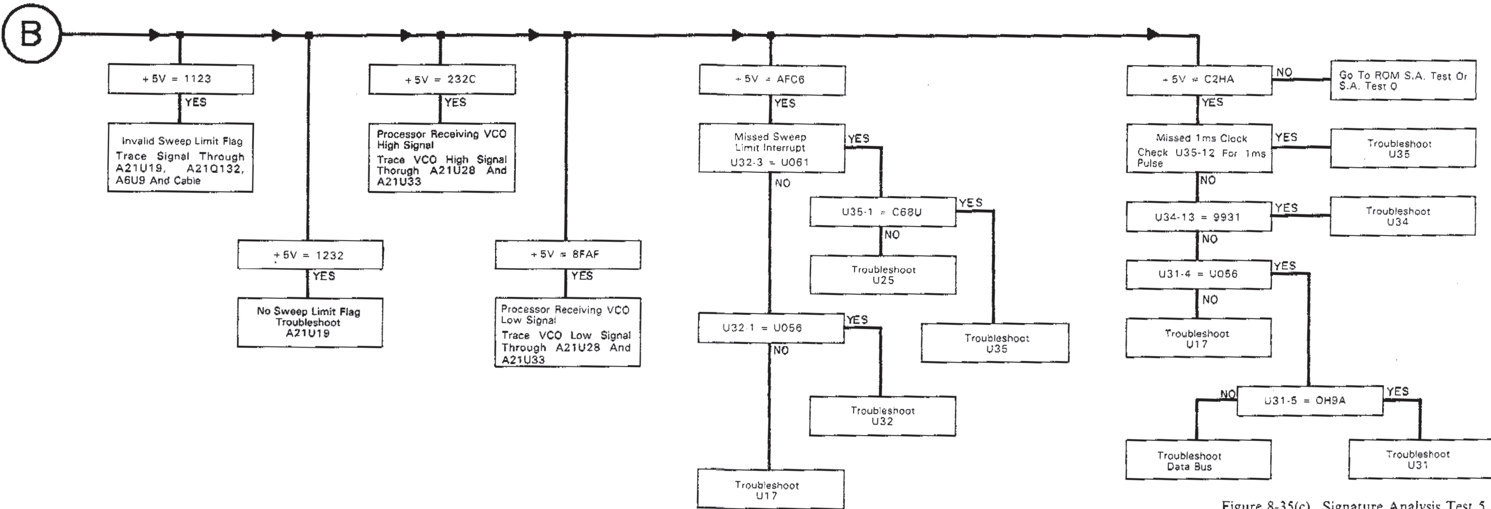
Figure 8-35(c). Signature Analysis Test 5.
