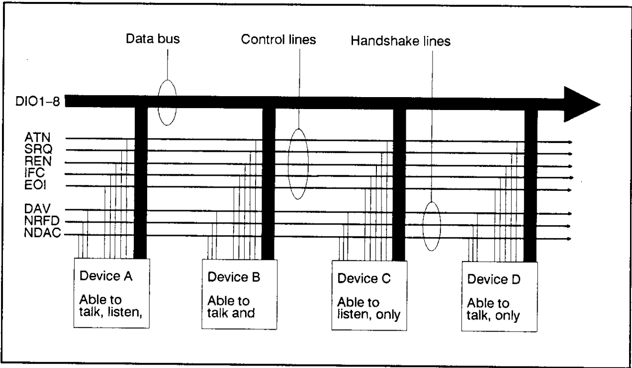
Figure 2-1. HP-IB Structure
