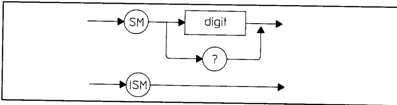
Figure 2-44. SM Syntax Diagram
