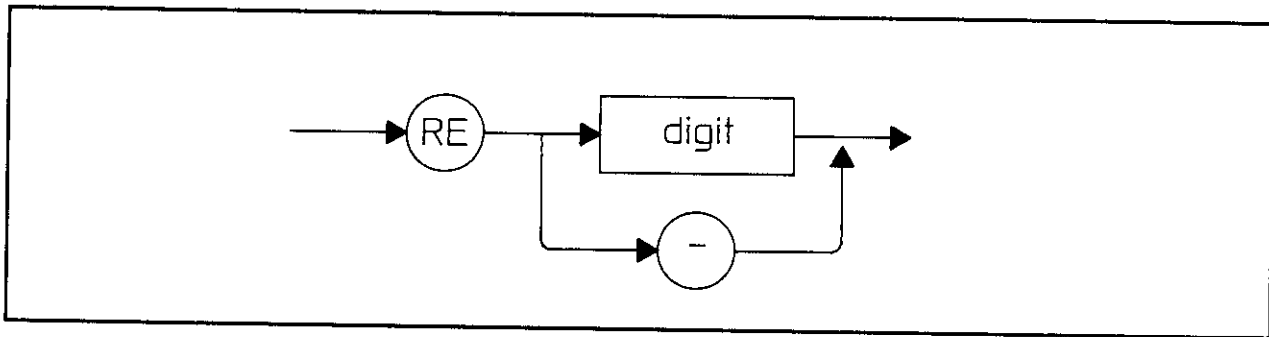
Figure 2-38. RE Syntax Diagram
