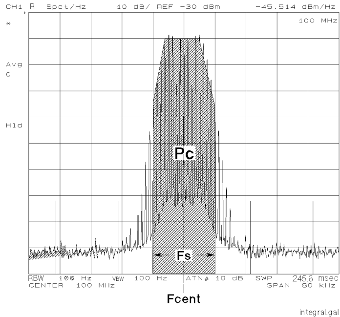
Figure 8-15. Integral Calculation of a Power
