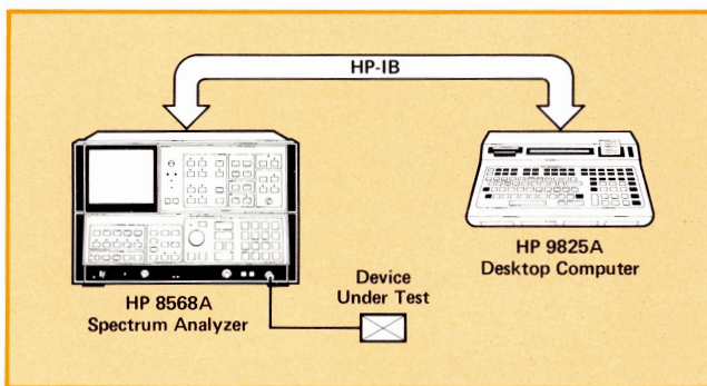
Figure 1. Measurement setup.
