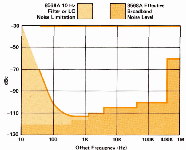
Figure 3. Discrete sideband measurement window.
