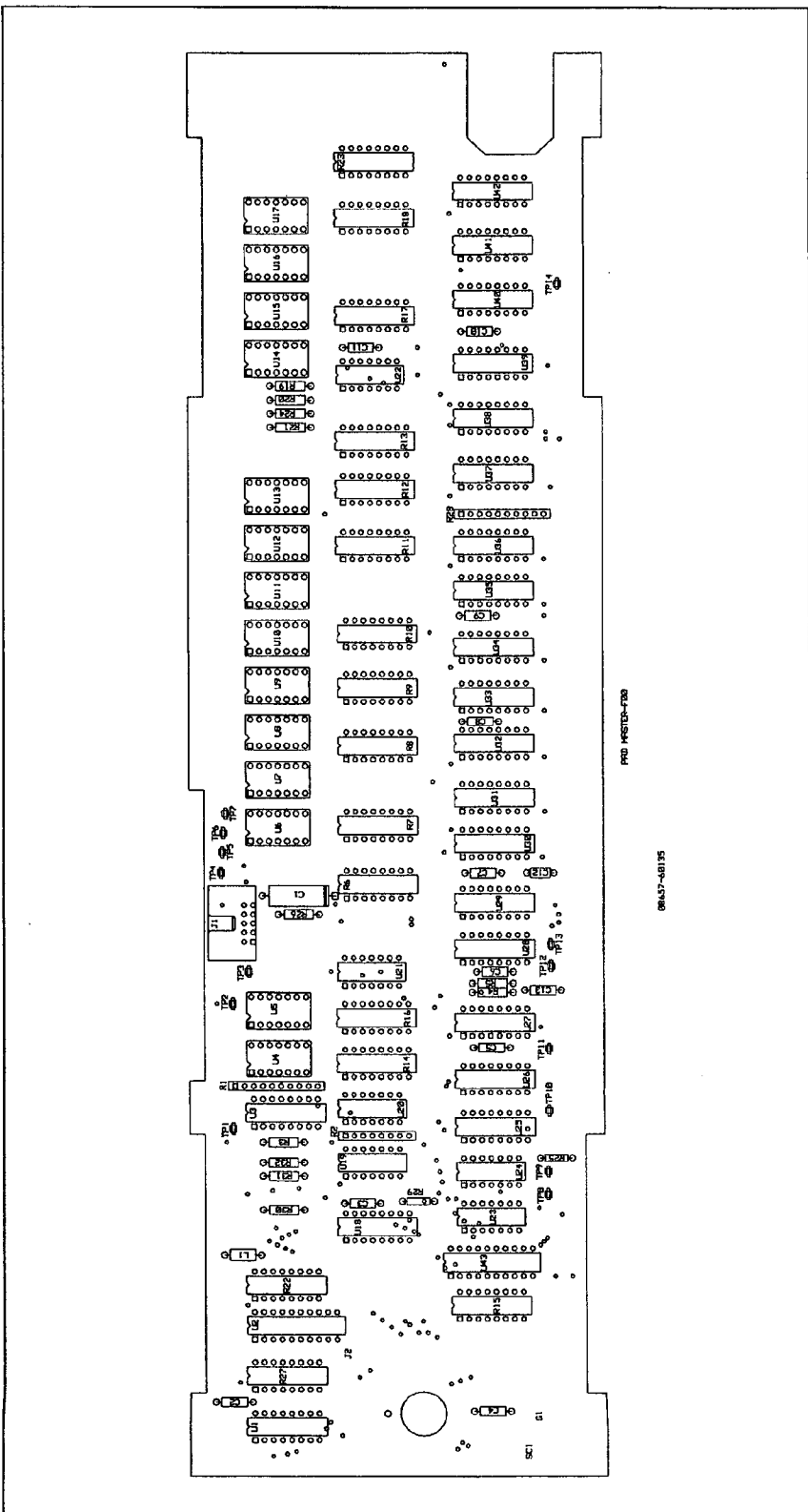
Component Locator
