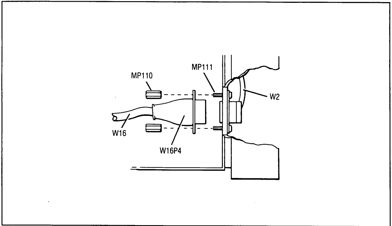
Figure 8-2. P/O A10/A11 Assembly Service Positioning.
