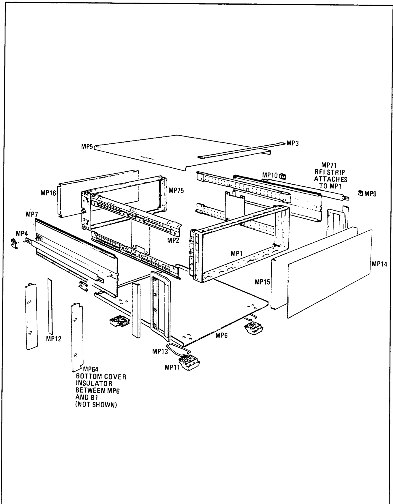
Figure 6-1. Cabinet Parts
