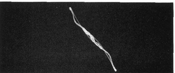
Square wave applied to two amplifiers, output of one on horizontal plates, output of other vertical plates for rapid comparison test. Nearly straight line obtained when amplifiers have nearly identical characteristics.
