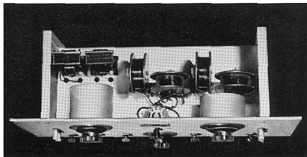
Views showing bottom and top of 320B chassis.
