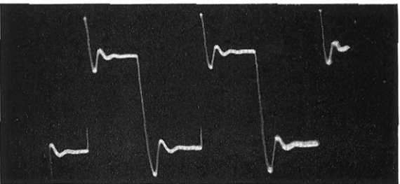
Square Wave test on a feedback amplifier showing amplification peak at 9 times square wave frequency. A normal frequency response measurement shows flat response from 20 cps to 20KC.)
