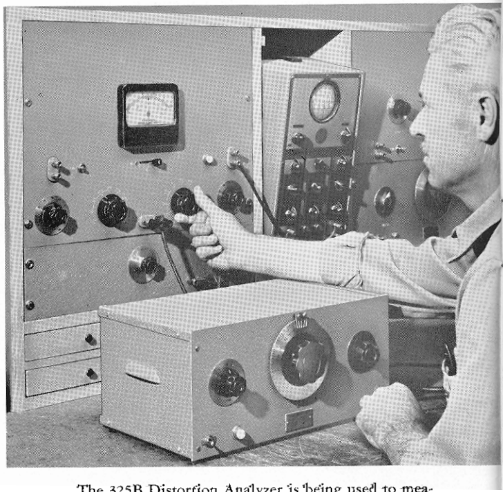
The 325B Distortion Analyzer is being used to measure the total harmonic distortion of a Model 200B on the production test bench.
