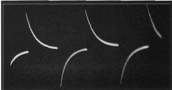
Square Wave Distortion from poor low-frequency sponse. (Phase shift of low frequency components wh always accompanies cut-off.)
