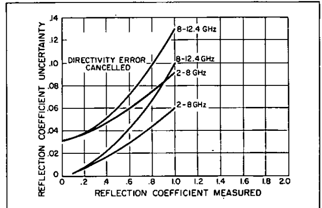
Reflection coefficient uncertainty including coupler directivity and when directivity is cancelled using a sliding load.
