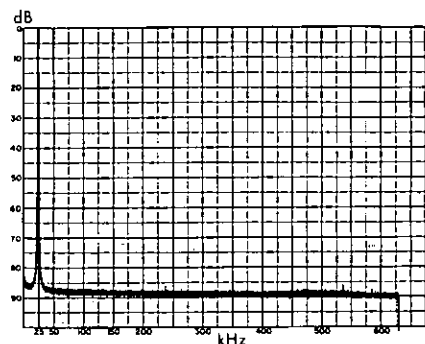
Figure 4. Recording of the 745A output, set at 25 kHz, as it is swept by the HP 3590A Wave Analyzer. The signal at zero frequency is the zero response of the 3590A.
