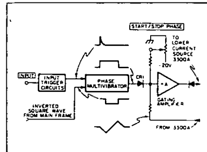
Figure 4. Block diagram of 3302A plug-in shown in single and multiple modes.
