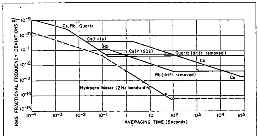
Figure 3. Short term stabilities of various frequency standards.
