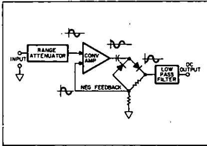
Figure 10. Typical ac/dc converter.
