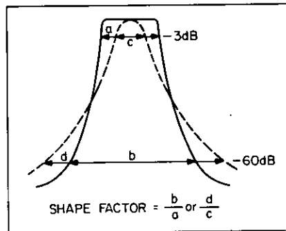
Figure 2. Shape factors for different wave analyzers.
