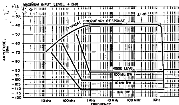
Figure 1. Noise level vs. Input Frequency.
