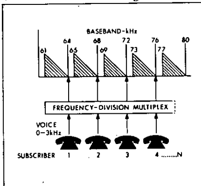
Figure 1. Voice channels are shown conventionally as triangles stacked by the multiplex (FDM) in the frequency spectrum. Each channel is 3 kHz-wide lower sideband (LSB) amplitude modulation on the appropriate multiplex carrier.
