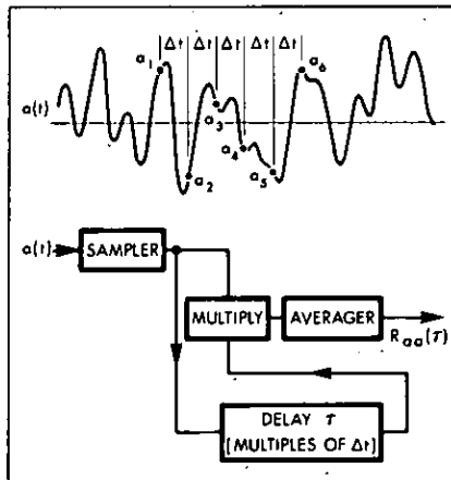
Figure 1. Computing autocorrelation function.
