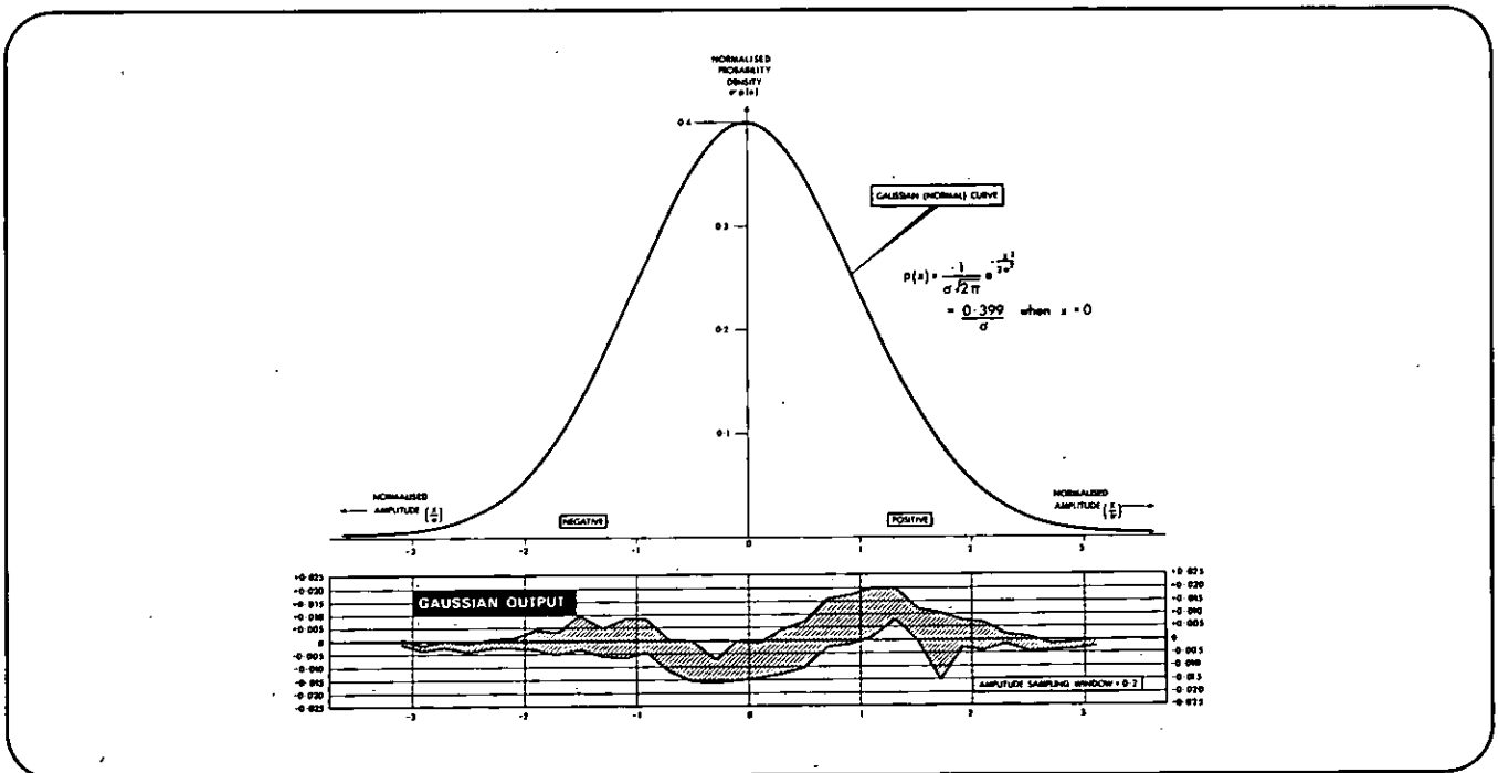
Envelope (shaded area) shows measured departures from the normal curve of 3722A Gaussian output p.d.f.'s for sequence lengths of 8,191 and greater.
