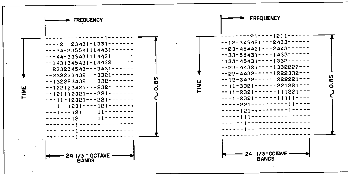
Figure 2. Sample Speech Patterns
