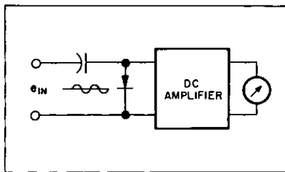
Figure 5. Peak-responding voltmeter.
