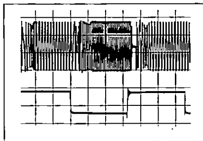
Figure 1. Switching speed, Model 5103A: 1.2 MHz to 2.7 MHz, 30 kHz switching rate. 5 \mu s/cm, 10 MHz Range.
