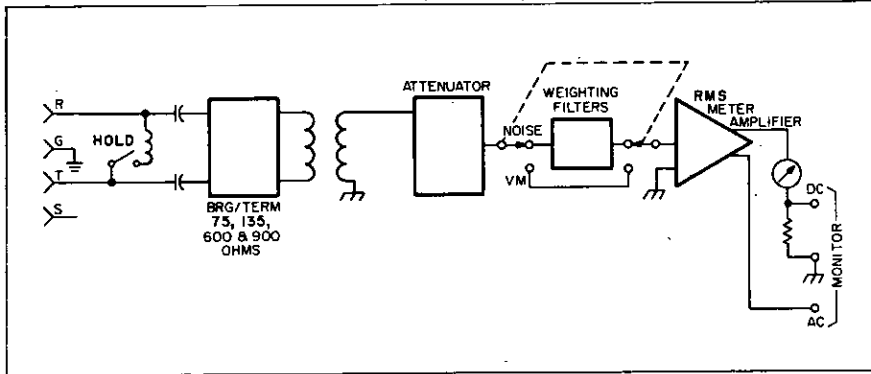
Figure 2. 3555B simplified block diagram.
