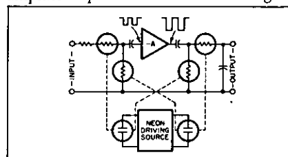
Figure 4. Amplifier with photoconductive modulator.
