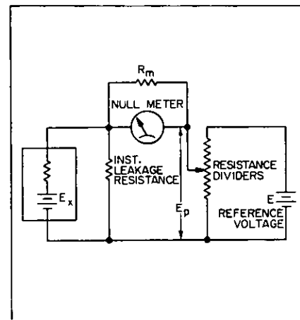
Figure 6. Classic differential voltage measurement.
