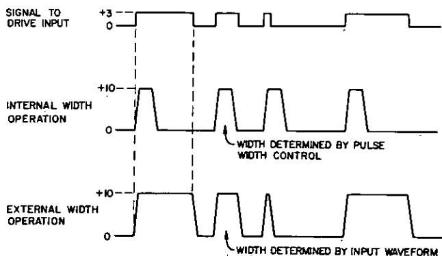
Figure 3. Middle waveform illustrates use of internal width control with pulses triggered by the top waveform. Lower waveform shows external width capability, using 1900 system as pulse amplifier with output pulse width determined by top waveform.
