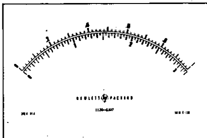
Figure 1. Scales for two different individually calibrated meters printed on one face by Hewlett-Packard's calibrator
