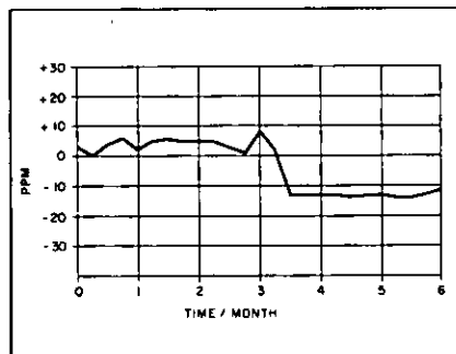
Figure 3. 6 month stability of a 745A reference supply.
