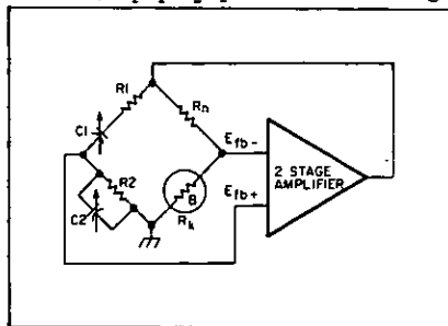
Figure 6. Basic HP Wien bridge RC oscillator circuit.
