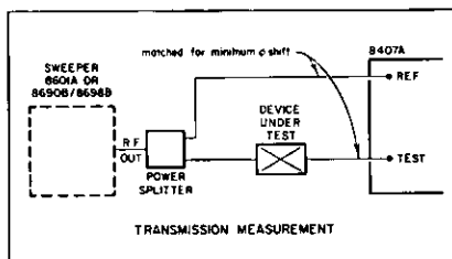
Figure 5. Transmission Measurement.
