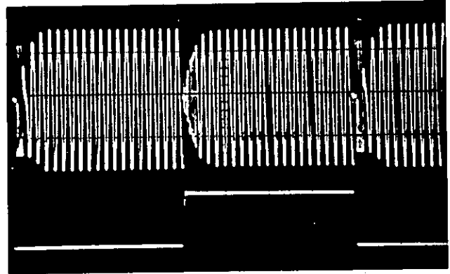
Figure 1. Synthesizer switching speed (25 \mu s/cm).
