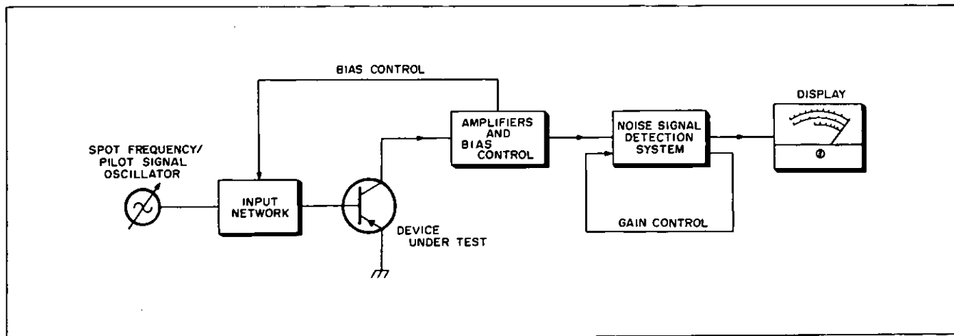
Figure 3. 4470A Basic Block Diagram
