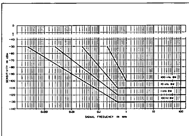
Figure 3. Noise level vs. Input Frequency.
