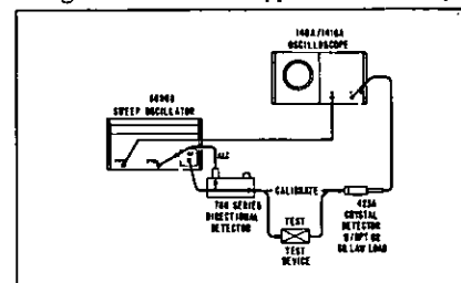
Figure 5. Typical Coaxial Setup for Square-Law Attenuation Measurement.
