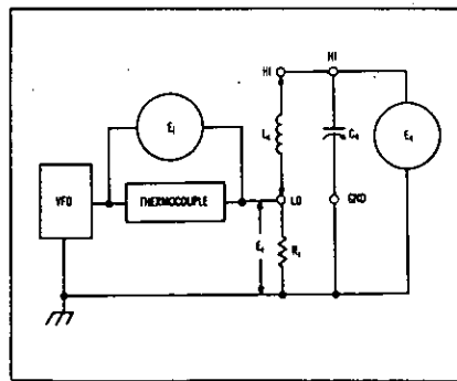
Figure 2. Q Meter.
