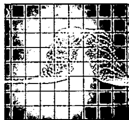
Jitter on delayed pulse in left photo eliminated at right by retriggering the delayed sweep. Sweep speed, 1 ns/div; delay, 5 \mu s.
