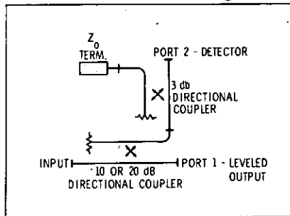
Figure 2. Super leveling with back-to-back waveguide coupler arrangement for extremely flat output.
