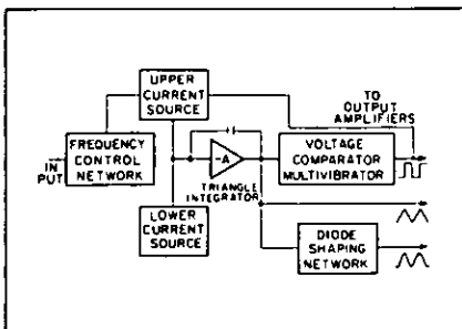
Figure 2. 3300A Function Generator.
