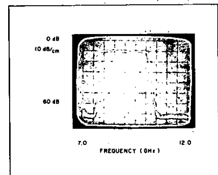
Figure 17. Swept-frequency display of an 8-10 GHz bandpass filter. Scale: 10 dB/cm vertical; 500 MHz/cm horizontal. Sweep speed: 0.01 second.
