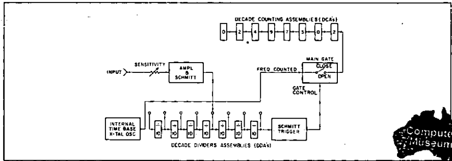
Figure 4. Function switch set to Period Average. Input signal controls gate for counting time base frequency.
