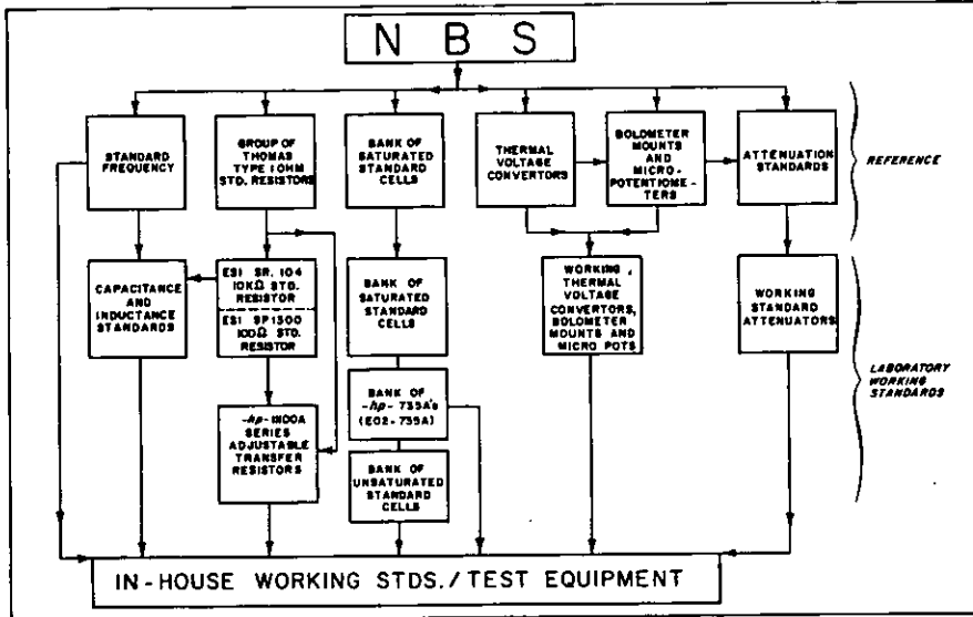
Figure 1. HP instrument traceability to NBS.
