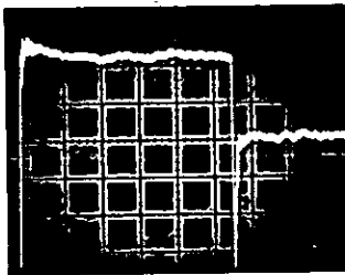
Impedance Mismatch: Reflection caused by cables of different impedance. With the vertical calibrated in .02 \rho/\text{div} and the first cable known to be 75\Omega , the second cable is quickly found to be 69\Omega using the TDR slide rule. From scope readout, the mismatch is located 55 ft down the 75\Omega cable.
