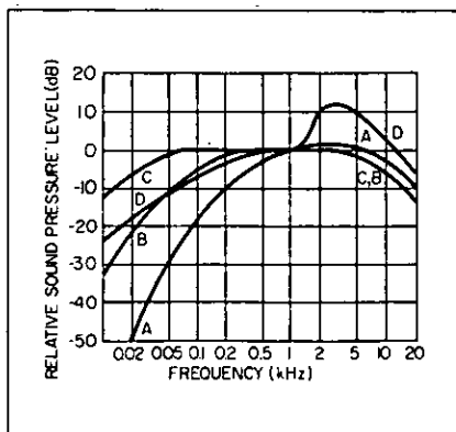
Figure 2. Frequency response curves.
