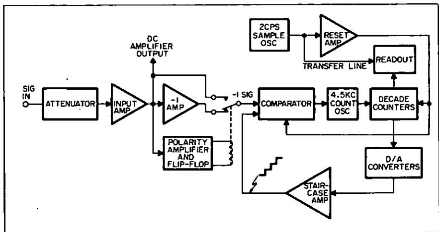
Figure 3. Block diagram of HP 3430A Digital Voltmeter.
