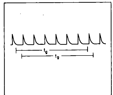
Figure 8. An error of \pm 1 count can occur because gate may open and close between input pulses. With gate open for upper t_g interval, 6 counts occur; 7 counts occur for lower interval.
