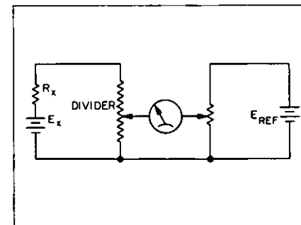
Figure 7. Potentiometric method of measuring unknown voltages.
