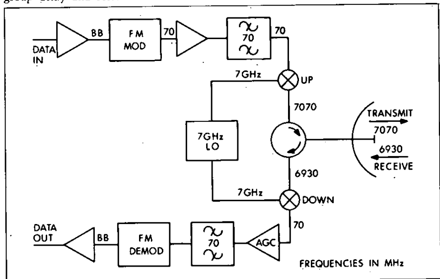
Figure 3. Simplified concept of a microwave link terminal. The main information encoder is the frequency modulator where input data is modulated by FM onto a 70 MHz carrier. This carrier, or IF, is up-converted to frequencies 3-10 GHz. In-coming transmissions are down-converted to 70 MHz and the data extracted in a frequency demodulator. Many links now in service have entirely solid-state electronics.
