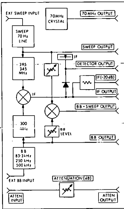
Figure 8. 3701A block diagram.
