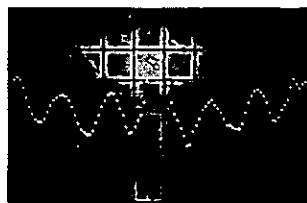
Crosscorrelation between noise in machine shop and noise from ventilation fan. Timescale 1 ms/mm. Peak centered on 47 ms shows propagation delay between microphone at fan and microphone in machine shop (approximately 50 ft separation).
