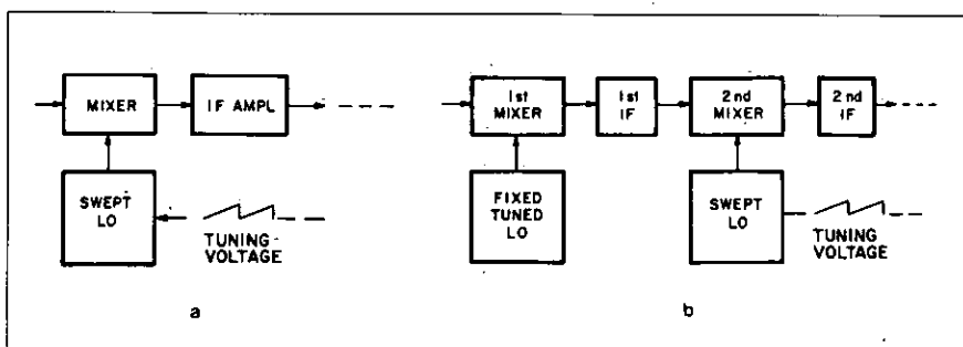
Figure 2. Two Methods of Obtaining Swept-Frequency Capability. a. Spectrum Analyzer using swept first LO. b. Spectrum Analyzer using swept second LO.
