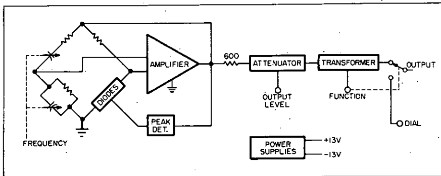
Figure 3. 236A block diagram.
