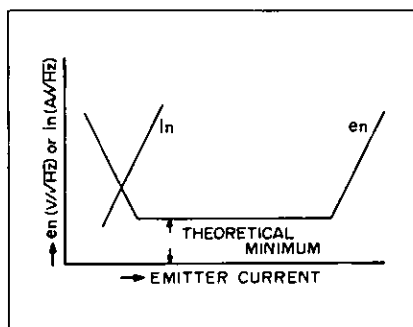
Figure 2. Theoretical Variation Of e_n, i_n
