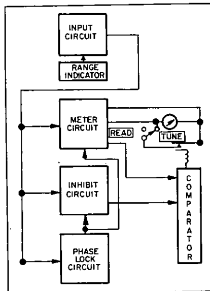
Figure 4. Block diagram of HP 3410A AC Microvoltmeter.
