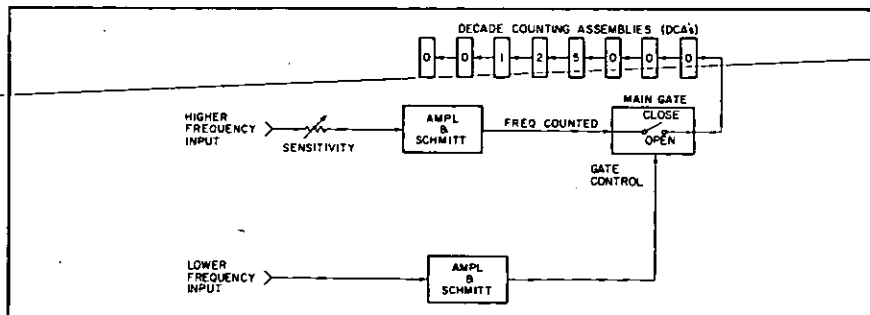
Figure 5. Ratio measurement. Function switch set to Period and time base switch to Ext. Lower frequency controls gate, while higher frequency replaces time base as counted frequency.
