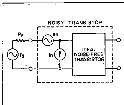
Figure 1. Transistor Noise Model
