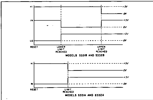
Figure 1. Control line outputs in MANUAL and HOLD modes.
