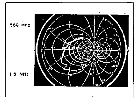
Figure 22. Swept-frequency display of impedance of a tunnel diode when it is biased in the negative impedance region.
