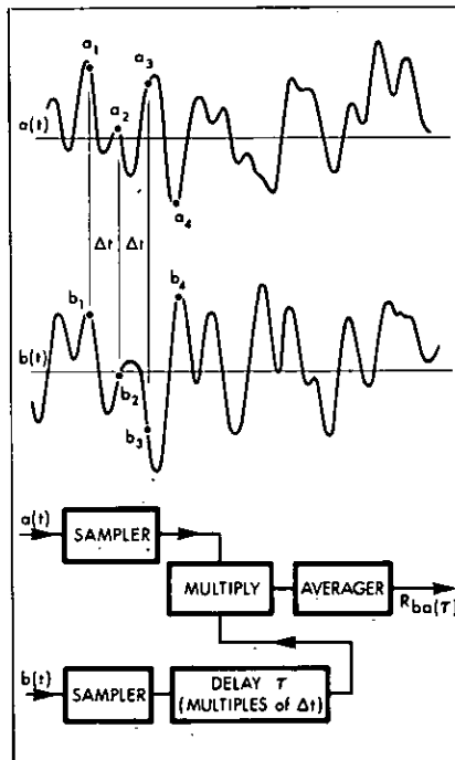
Figure 3. Computing crosscorrelation function.
