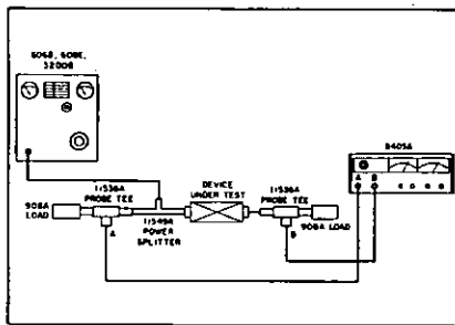
Figure 13. Transmission tests for phase and amplitude response (attenuation or gain) of a test device can be made over a dynamic range greater than 90 dB.
