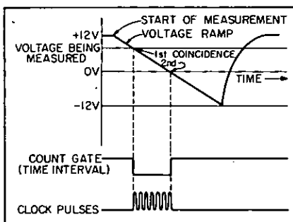
Figure 1. Voltage-to-time conversion.
