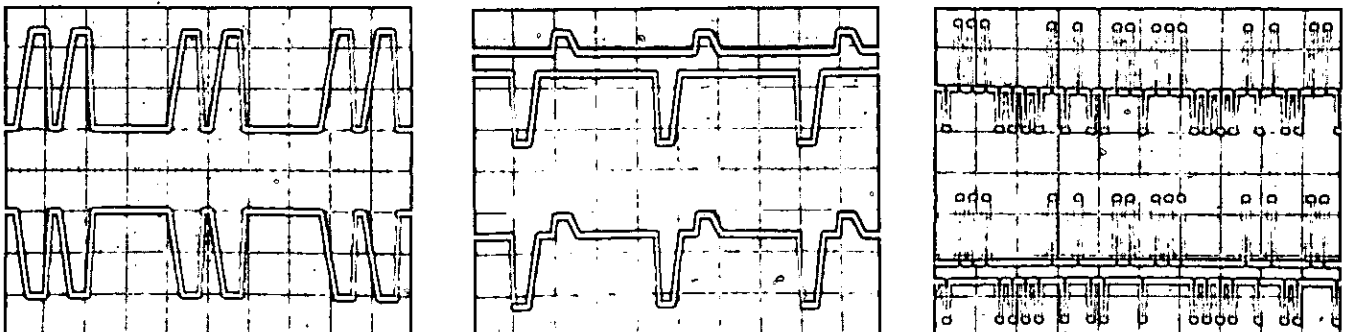
Figure 1. (a) Separate output in double pulse mode. (b) Combined and separate non-simultaneous outputs. (c) A/B gating of combined and separate outputs.
