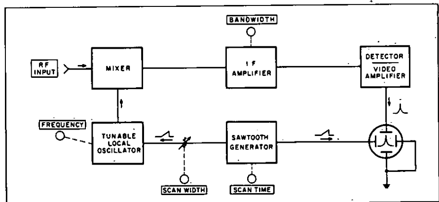
Figure 1. Simplified Spectrum Analyzer of the Swept-Receiver Design.
