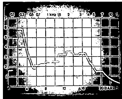
Figure 3. Loudness spectrum.
