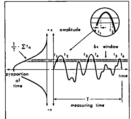
Figure 4. Measuring pdf of random signal.
