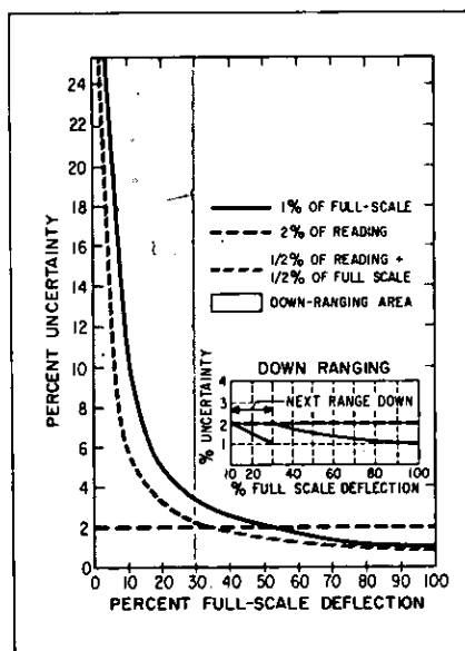
Figure 8. Percent uncertainty for three methods of specifying accuracy.
