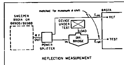
Figure 8. Reflection Measurement.
