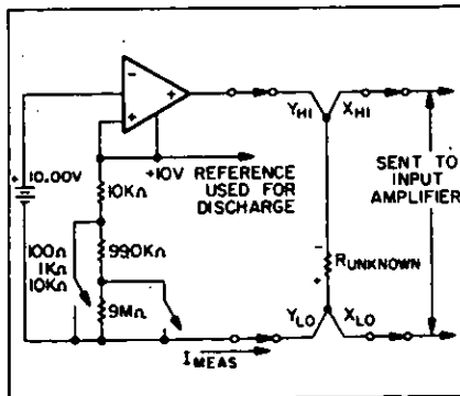
Figure 9. Ohms converter for the 3450A.
