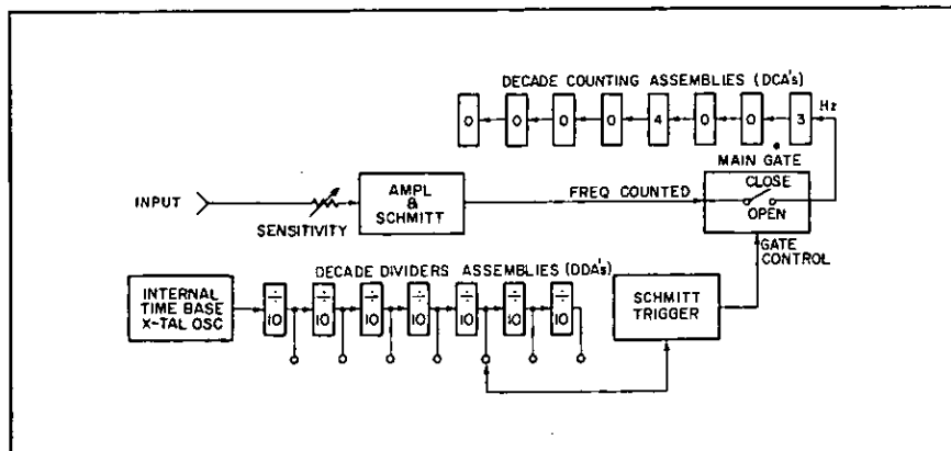
Figure 2. Function switch set to Frequency and gate time selected by time base switch.
