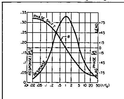
Figure 7. Characteristics of frequency-determining network.
