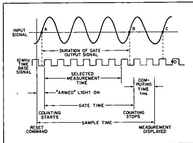
Figure 2. The Measurement Cycle.
