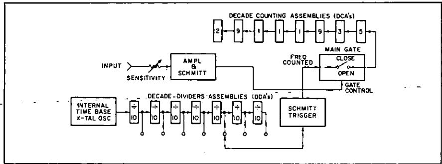
Figure 3. Function switch set to Period and counted frequency selected by time base switch.
