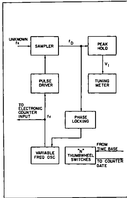
Figure 7. Frequency measurement with HP 5257A Transfer Oscillator using new transfer oscillator principle; counter measures sampling frequency of sampler.
