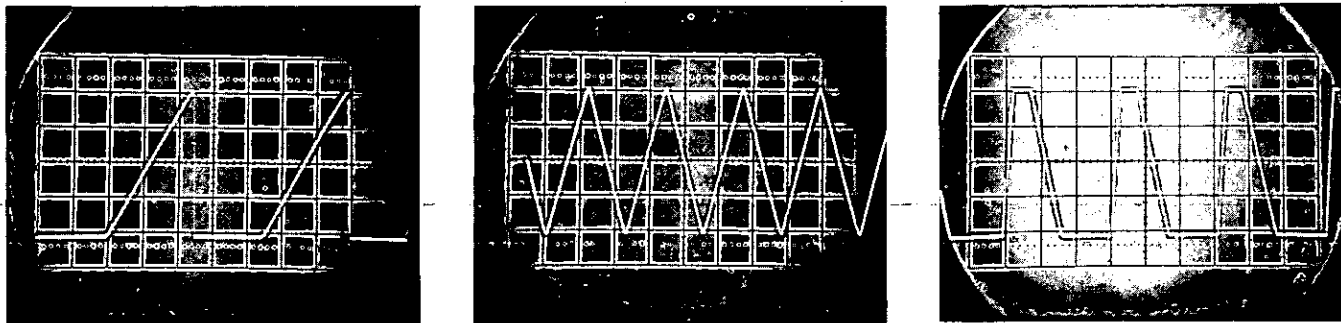
Figure 1. Typical Waveforms produced by the 8002A. Variable Rise and Fall Time Pulse Generator.
