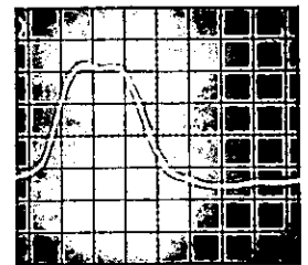
Jitter on delayed pulse in left photo eliminated at right by retriggering the delayed sweep. Sweep speed, 1 ns/div; delay, 5 \mu s.
