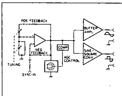
Figure 5. Block diagram of 209A Sine and Square Wave Oscillator.
