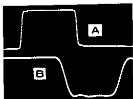
Figure 2. (A) Input Pulse to HP 462A (5 mV peak to peak). (B) Output Pulse of HP 462A (500 mV peak to peak). Gain control is set in 40 dB position. Sweep speed is 5 ns/cm.
