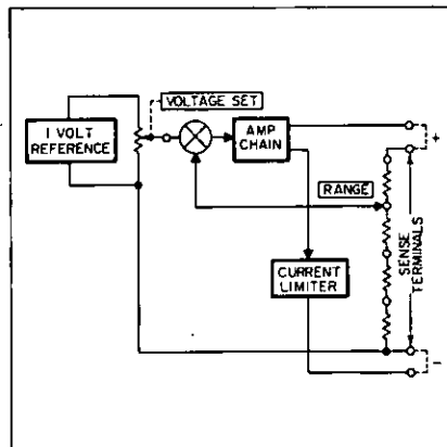
Figure 5. HP simplified dc standards diagram.
