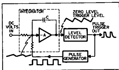
Figure 4. Voltage-to-frequency conversion.
