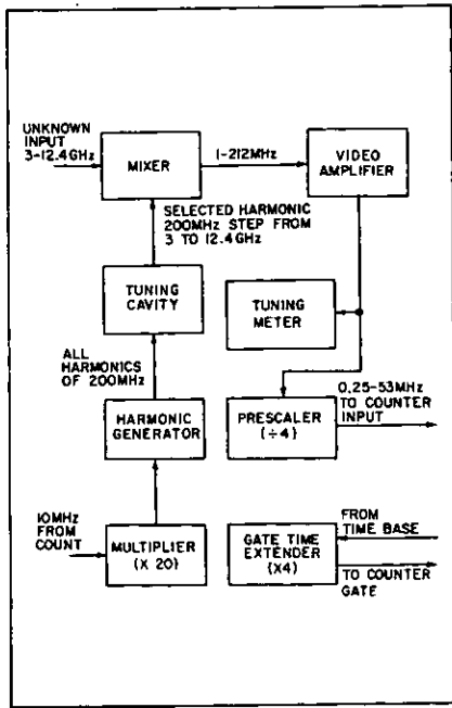
Figure 6. Frequency measurement with heterodyne converter; counter measures difference frequency (diagram is of HP 5255A Converter).
