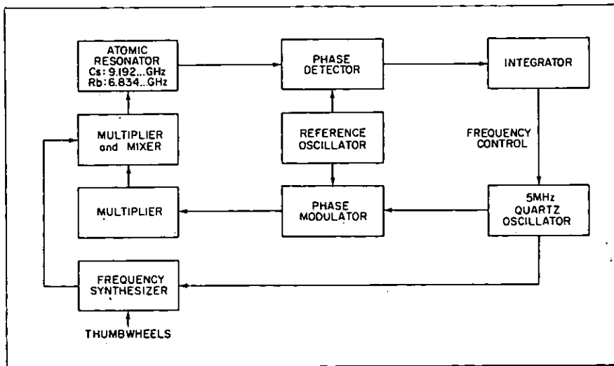
Figure 1. Typical atomic standard phase-lock loop system.
