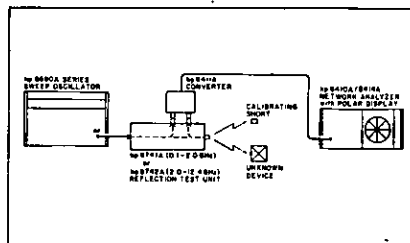
Figure 20. Reflectometer setup for Smith Chart impedance measurements. Readout of both the reflection coefficient magnitude and angle can also be made directly from polar display unit.
