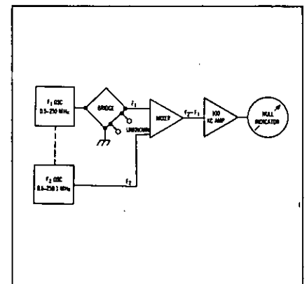
Figure 3. RX Meter.
