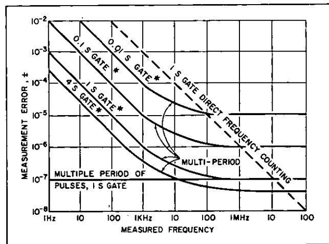
Figure 1. Accuracy vs. Gate Time for period measurement (5323A) and conventional direct frequency counting. Time base errors, which would affect both methods equally, are excluded. Multi-period plots are for 100 mV sine wave input with 40 dB signal-to-noise ratio, and are statistical (99% confidence level).
