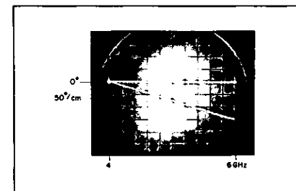
Figure 27. Linear phase shift indicates constant group delay for frequencies between 4 and 6 GHz. 150° phase shift in 2 GHz gives group delay of 11.9 nanoseconds.
