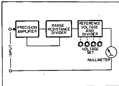
Figure 8. Simplified diagram of dc standard, differential voltmeter in differential voltmeter mode.
