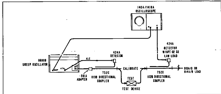
Figure 4. Swept attenuation system for measurements up to 40 dB with oscilloscope.
