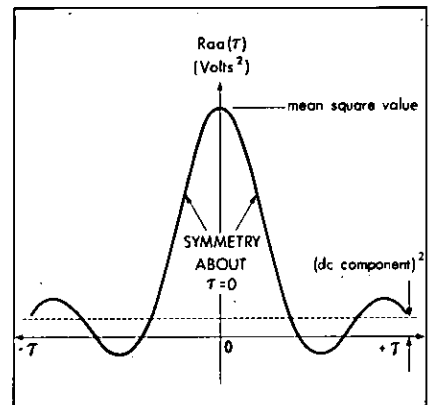
Figure 2. Autocorrelation function of random signal.
