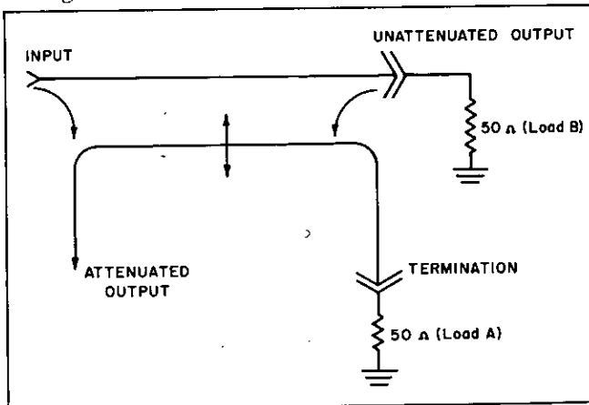
Figure 1. With loads A and B in place the instrument is an attenuator. With load A only, the instrument is a variable directional coupler.
