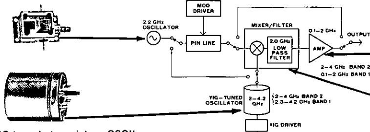
8699B Block Diagram
