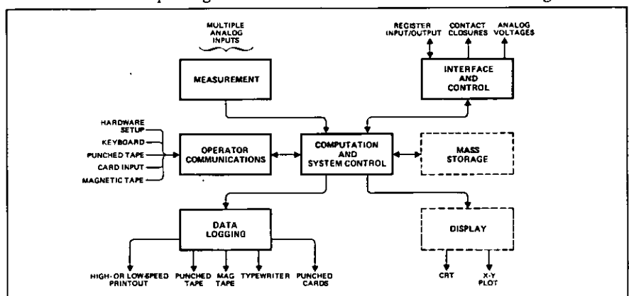
Hardware and computer-controlled data acquisition system composite block diagram.
