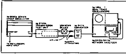
Figure 18. Typical test setup for measuring swept or CW phase shift and attenuation (gain) through a device.
