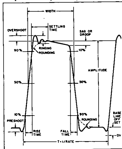
Figure 2. Test pulse description in terms of primary characteristics.
