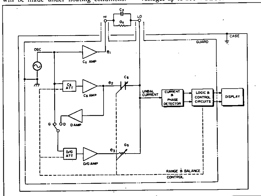
Figure 1. Simplified block diagram of HP 4270A Automatic Capacitance Bridge
