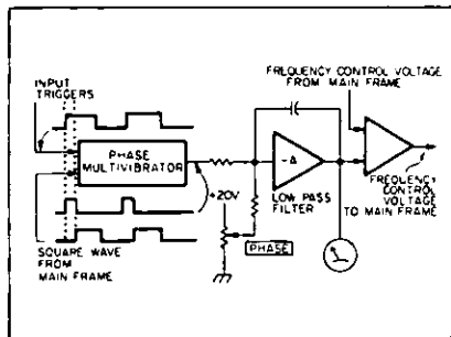
Figure 3. Block diagram of 3302A plug-in phase lock mode.
