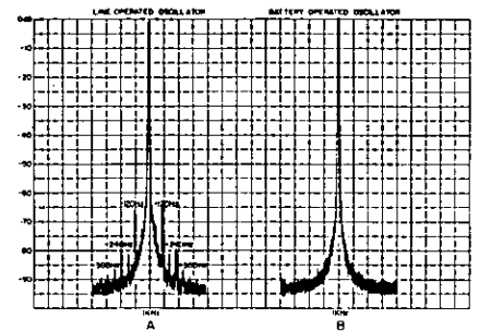
Figure 6. Line-frequency related FM sideband detection is accomplished by using the 3590A's 10 Hz bandwidth. Note that no sidebands are generated by the analyzer.
