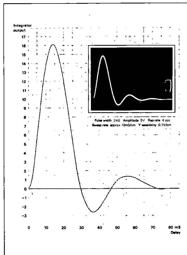
Impulse response of LC filter measured using 3722A option H01. Photo inset shows filter's response to a 2 ms pulse.
