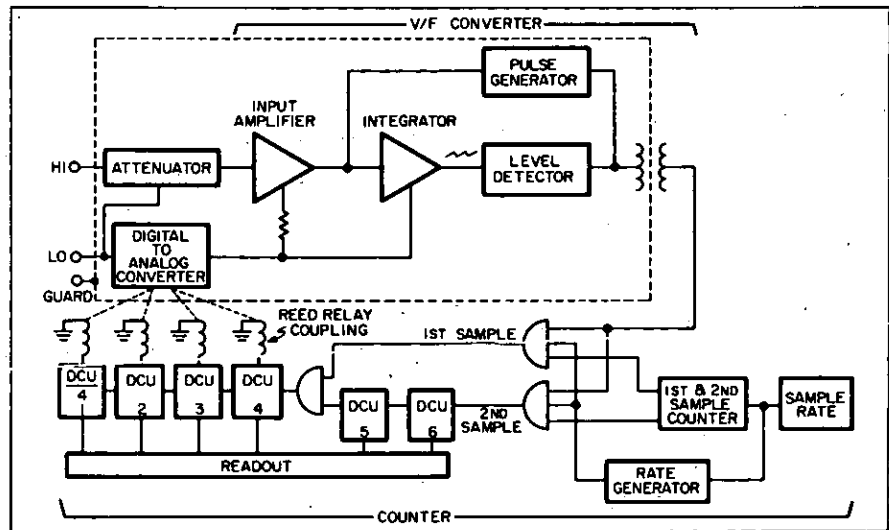
Figure 6. Block diagram of HP 3460B DVM.
