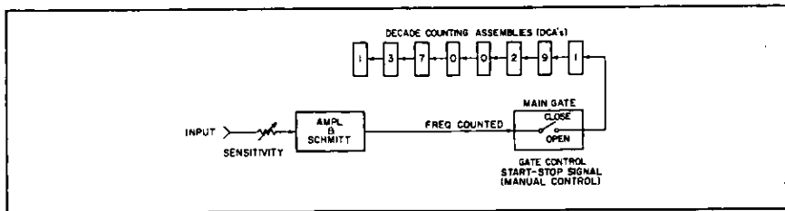
Figure 1. Function switch set to manual Start and Stop for totalizing.
