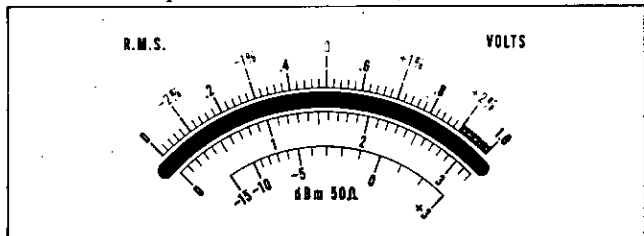
HP 652A expanded meter scale
