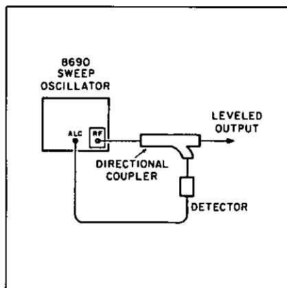
Figure 1. Basic closed-loop leveling system.
