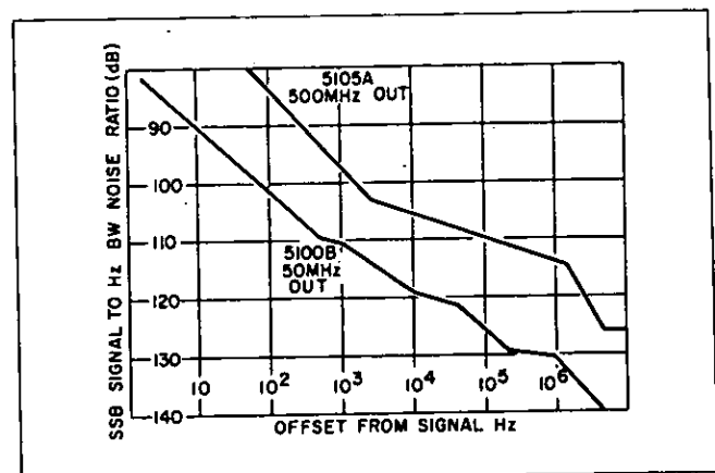
Figure 2. Composite phase noise plot for Hewlett-Packard synthesizer.
