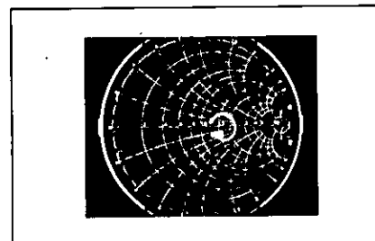
Figure 10. Antenna Complex Impedance—An FM antenna was swept over its usable range of 88 to 108 MHz, using the 8414A display with Smith chart overlay. 50-ohm input Z is desired (the exact center of the display) but the antenna varies from inductive to capacitive over the sweep range. Values of complex impedance can be read directly off the Smith chart.
