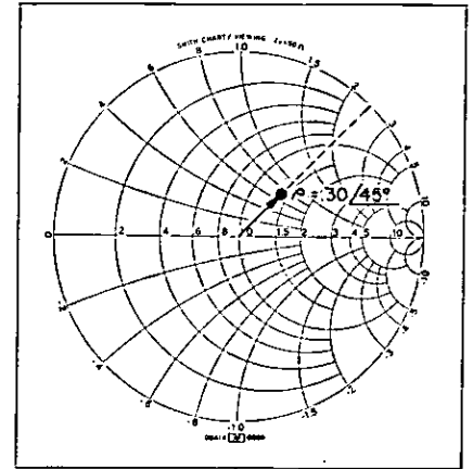
Figure 21. Plot of the impedance for a reflection coefficient of known magnitude and phase \rho = 0.30/45^\circ .
