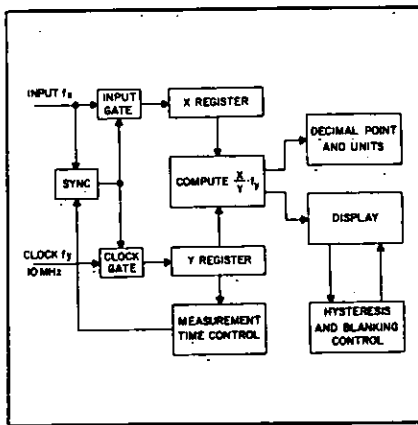
Figure 10. 5323A Automatic Counter. Computing circuits divide the number of input cycles (X) by the number of clock periods (Y) and multiply by f_y = 10^7 to find the unknown frequency f_x . Other IC's determine the measurement units, position the decimal point, blank insignificant digits, and apply hysteresis to prevent display jitter.
