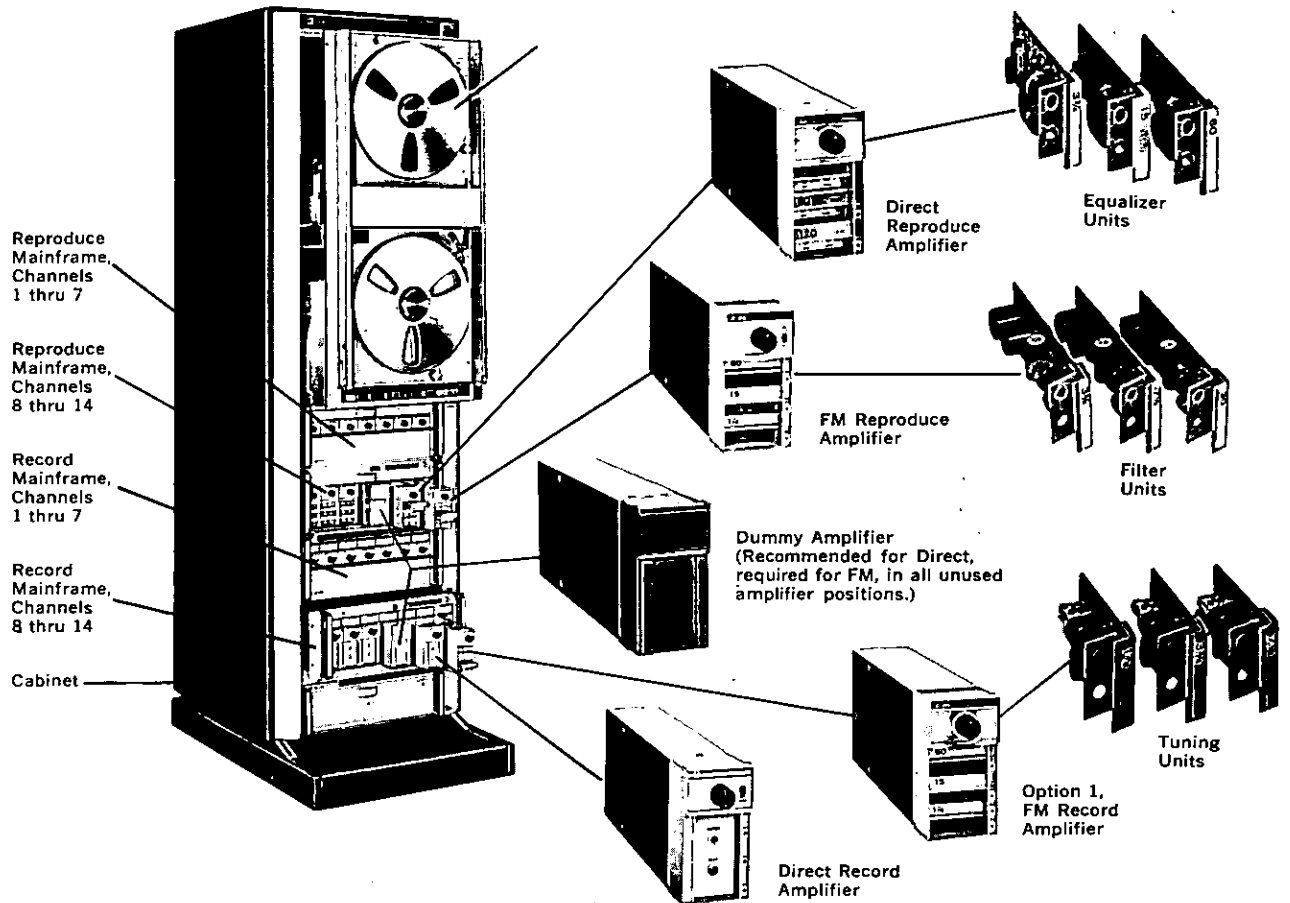
Figure 2. Modular system configuration.
