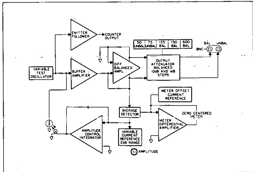
Figure 9. Block diagram of the balanced 654A Oscillator.
