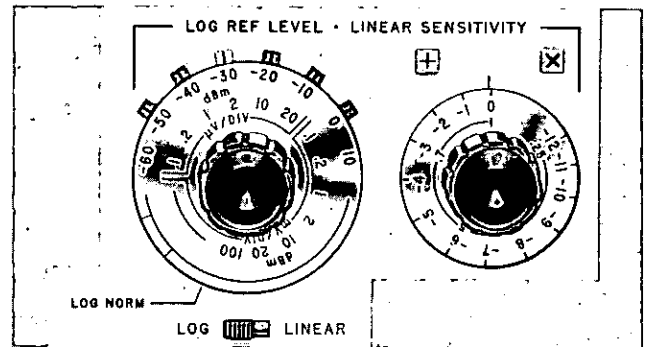
Figure 3. Settings of the INPUT ATTENUATOR and LOG REFERENCE LEVEL controls determine the scale factor for absolute amplitude calibration. Here, LOG is selected and the "+" lamp lights to indicate that LOG REFERENCE LEVEL is the sum of the black color-coded dial readings; i.e., LOG REF = -30 dBm + 0 dBm = -30 dBm.
