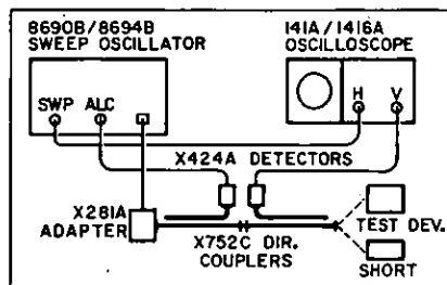
Figure 3. Typical Waveguide Reflectometer.
