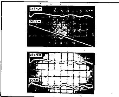
Figure 19a. Insertion phase and attenuation of a PIN modulator showing both amplitude frequency response and the linear phase shift due to excess electrical length.
