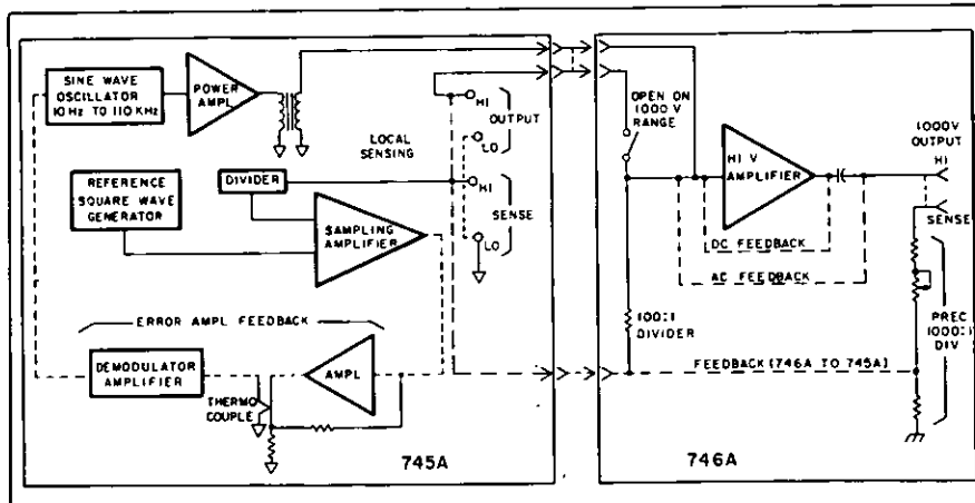
Figure 2. 745A, 746A AC calibrator block diagram.
