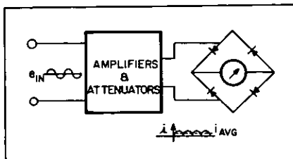
Figure 3. Average-responding voltmeter.
