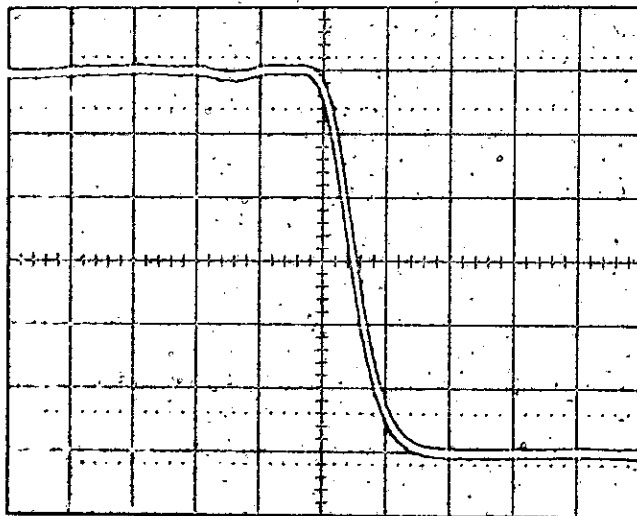
The clean, fast rise of the 220A's output delivers -5 V into 50 ohms.
