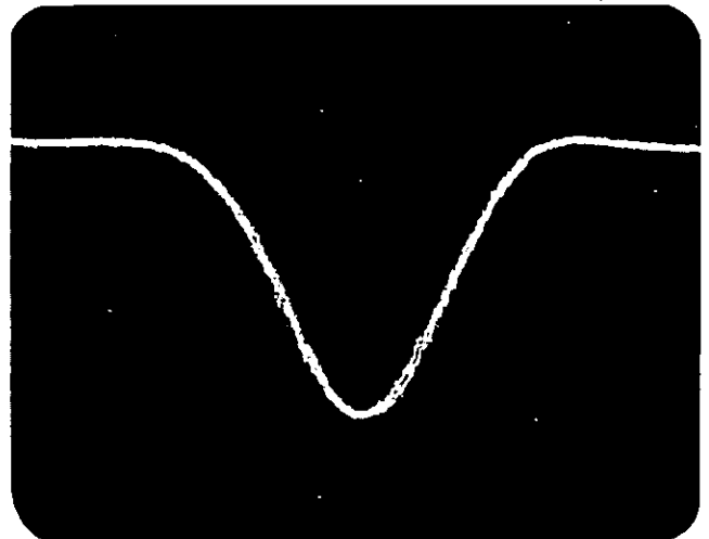
CRT display using Model 1815A/1817A/1106A TDR system slows the reflection from HP Model 874B Susceptance Standard set at 1 pF equivalent capacitive discontinuity. Scale: 20 ps/div horizontal, 0.1 p/div vertical.
