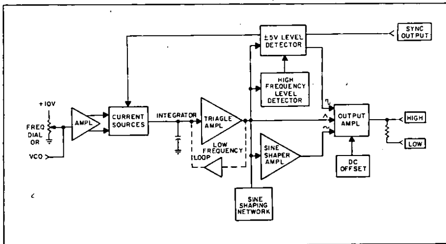
Figure 1. Block diagram of 3310A Function Generator.
