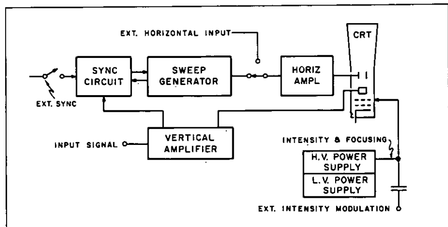
Figure 2. Oscilloscope block diagram.
