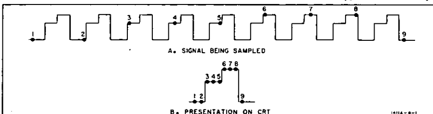
Figure 4. The sampling oscilloscope reconstructs the test signal by taking up to 1000 samples.
