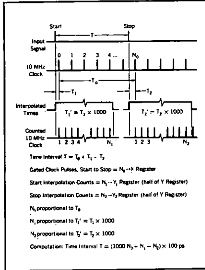
Figure 11. Time intervals measured by 5360A Computing Counter.
