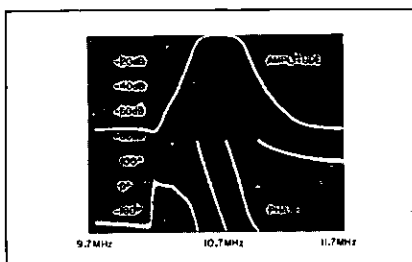
Figure 3. Phase and amplitude response of an LC filter displayed on an oscilloscope.
