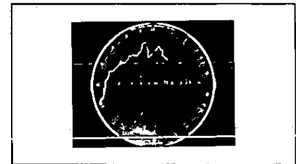
Figure 26. Swept-frequency display of s_{11} of a transistor with Smith Chart overlay for direct impedance readout. Frequency range: 300 MHz to 700 MHz.
