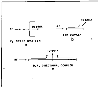
Figure 16. Reference and test channels for the network analyzer may be obtained using various methods such as a) power splitters, b) 3-dB couplers, c) dual directional or back-to-back couplers. The second coupler in c would be turned around for transmission measurements.
