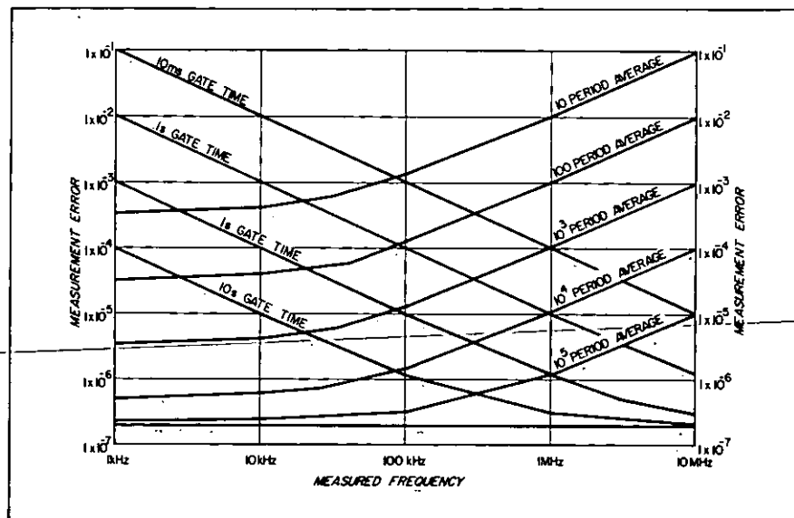
Figure 9. Comparison of error vs measured frequency for frequency measurements (plots labeled "gate time") and period measurements. Example is for HP 5325B Counter. Total time base error assumed to be 2 \times 10^{-7} . Note that low frequencies are best measured by multiple period averaging.
