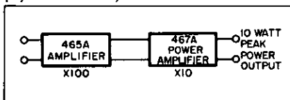
Figure 1. Cascading the HP 467A Power Amplifier with the HP 465A Amplifier results in a stable 60 dB amplifier with 10 M \Omega input impedance and 10 W peak-power output.
