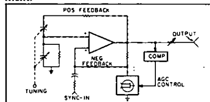
Figure 8. Block diagram of the 204C Oscillator.
