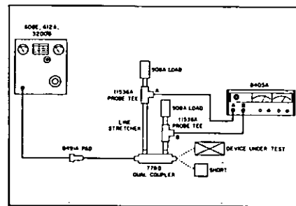
Figure 14. Amplitude and phase of reflected signal from test device can be measured directly using a dual directional coupler.
