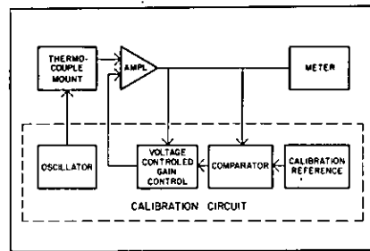
Figure 2. 437A Calibration Circuit. An audio oscillator delivers a precise 10 kHz signal to the mount. The amplified output voltage is then compared to a calibration reference. Any difference appears as an error signal which actuates a voltage controlled gain control to compensate the instrument gain.
