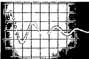
Impulse response of under-damped servo, obtained by crosscorrelation method.
