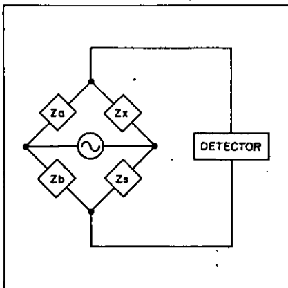
Figure 1. Generalized Bridge Circuit
