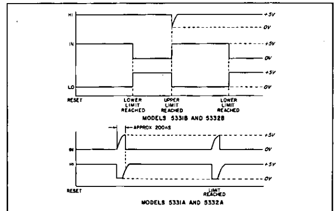
Figure 2. Control line outputs in RECYCLE mode.
