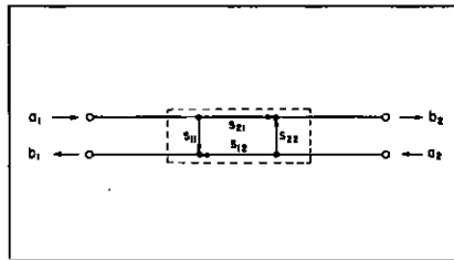
Figure 25. S-parameter representation of a two-port microwave device.
