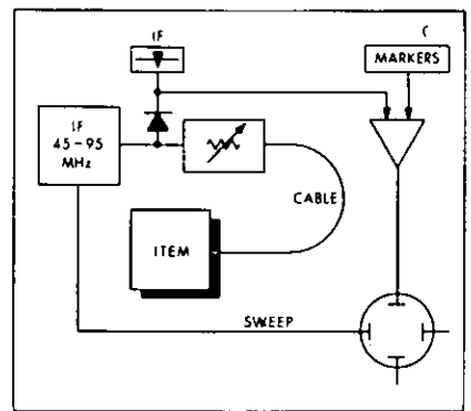
Figure 7. Long cable method of return loss measurement has IF level second-harmonic balanced detector, two-way attenuator and 15 ft. or more of 75 ohm cable. Ripples caused by VSWR of item are noted on display, the item is disconnected, and ripples caused by open-ended cable are attenuated to match the previous ripples. Twice the attenuation applied is the return loss figure.
