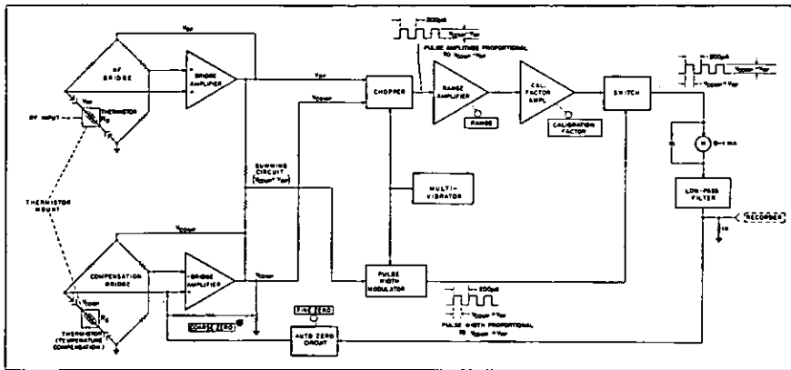
Figure 3. Block diagram of HP 432A Power Meter. Dual bridge provides proper bias to thermistor mount to correct for temperature variation and reduce zero drift.
