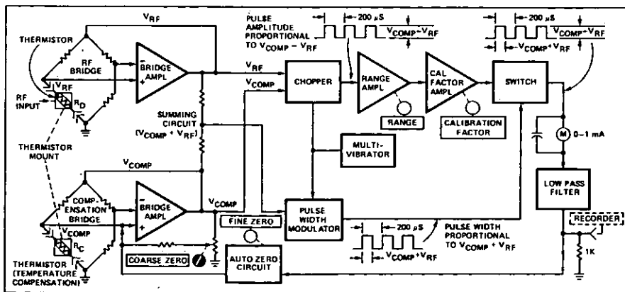
Figure 4. Block diagram of 432A Power Meter. Dual bridge provides proper bias to thermistor mount to correct for temperature variation and reduce zero drift.
