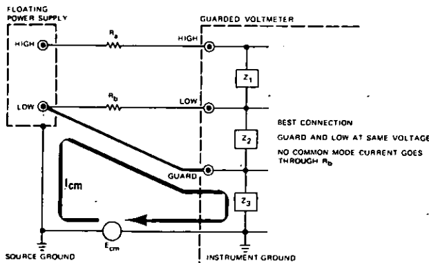
Figure 5 — Best connection—guard connected to low at source
