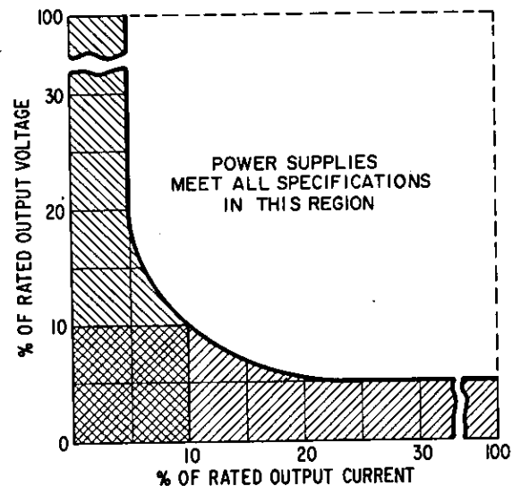
POWER SUPPLY OUTPUT RESTRICTIONS AS A FUNCTION OF LOADING (REFER TO NOTE 6 ON SPECIFICATION PAGES)
