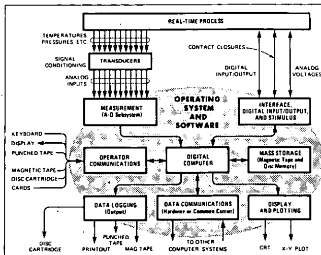
Automatic measurement and control system major functions
