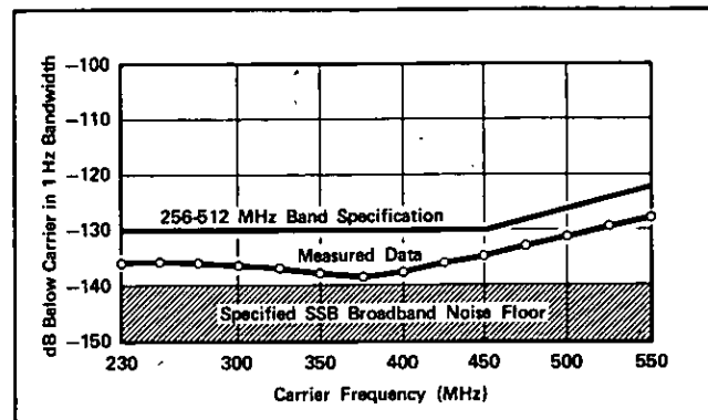
Specified Signal to Phase Noise Ratio at 20 KHz Offset vs. Carrier Frequency.
