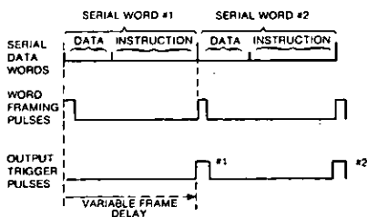
Figure 2. Since frame delay and bit pattern can be user-defined, pattern recognition triggering on serial data can be set to occur when the instruction portion of a serial word matches a user-selected bit pattern.
