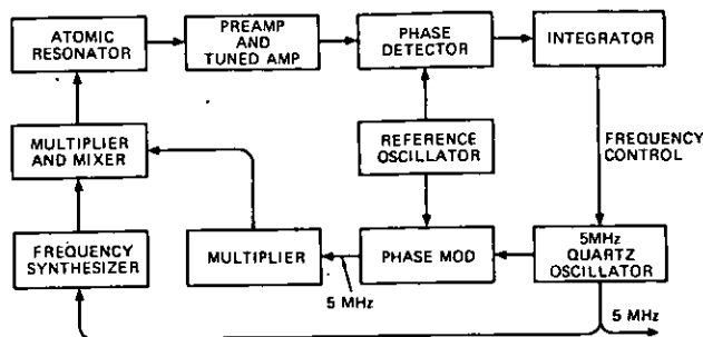
Figure 1. Block diagram of atomic frequency standards.
