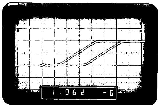
For increased accuracy, the scope is placed in the Delayed Sweep mode to display the two intensified traces alternately. When the two traces are made to coincide using the DEC \leftrightarrow INC controls, maximum accuracy is achieved: (1.962 \mu s, \pm 0.63\% ).
