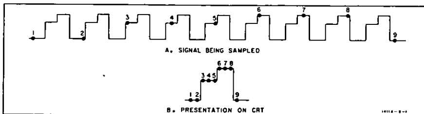
Figure 6. Sampling scope technique reconstructs waveform from consecutive samples.
