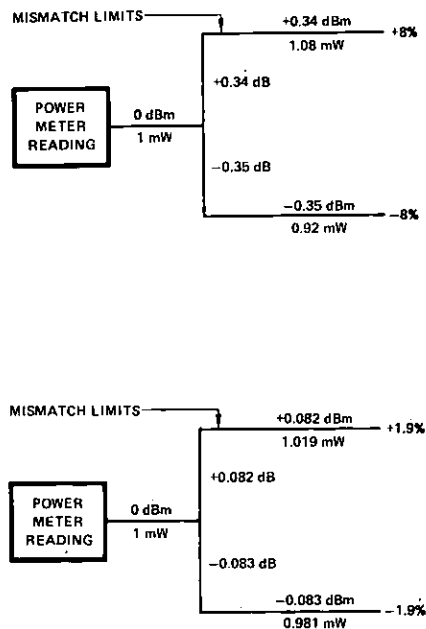
Figure 3. Limits of mismatch uncertainty when VSWR of source is 1.5 and VSWR of power meter is 1.1.
