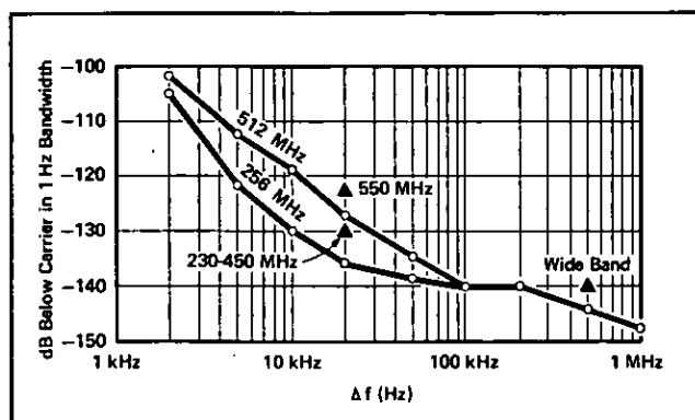
Measured SSB Noise vs. Offset from Carrier. Markers indicate specified limits.
