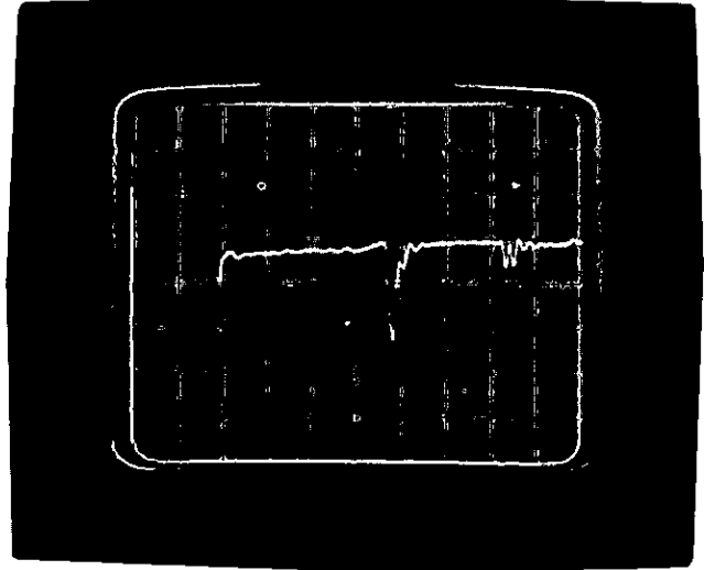
The 1818A provides a system profile which includes quantitative and qualitative information about a transmission cable's impedance loss, rise time, electrical length, and location of discontinuities in a single measurement.
