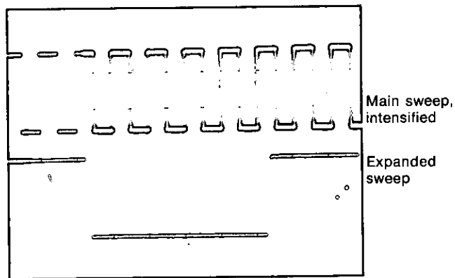
Double exposure shows intensified main sweep with location of intensified portion (top trace). Bottom trace shows expanded sweep.
