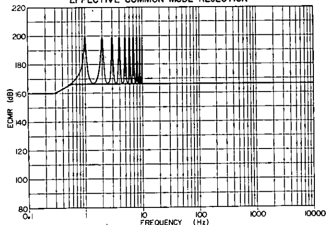
EFFECTIVE COMMON MODE REJECTION
