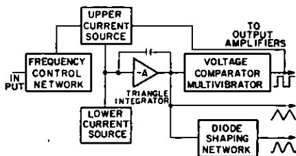
Figure 1. Block diagram typical function generator.
