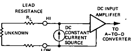
Figure 2 — Simple two-wire ohms converter
