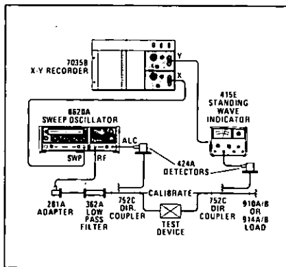
Figure 2. Swept attenuation system for measurements up to 30 dB.
