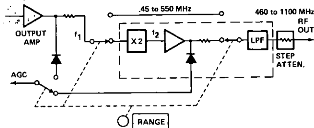
Figure 1. Internal Doubler Block Diagram
