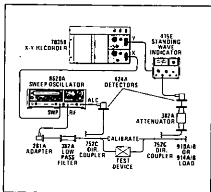
Figure 4. RF pre-insertion technique for swept attenuation measurements.
