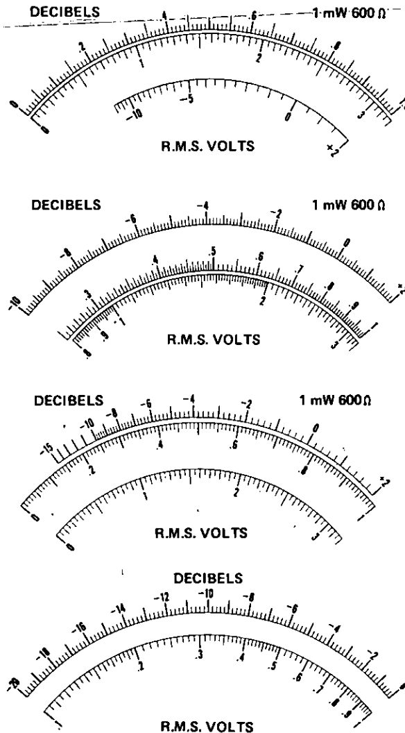
Figure 1. Four different types of meter scales available. (a) Linear 0–3 V and 0–10 V scales plus a dB scale. (b) Linear dB scale plus non-linear (logarithmic) voltage scales. (c) dB scale placed on larger arc for greater resolution. (d) Linear –20 to 0 dB scale useful for acoustical and communications applications.
