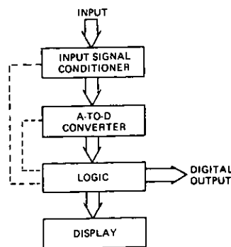
Figure 1 — Basic building blocks of a DVM
