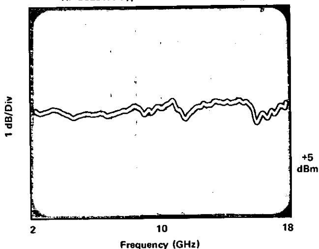
HP 86290A Typical Levelled Power Output
