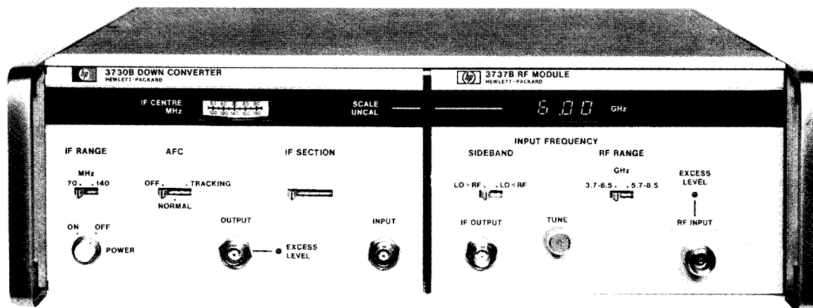
HP 3730B Option 010 Down Converter mainframe with HP 3737B RF Module plug-in
