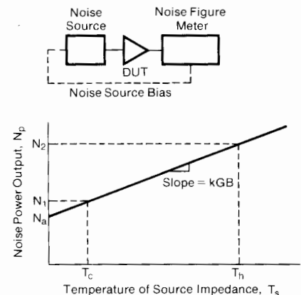
Figure 3. Available noise power and noise figure measurement.
