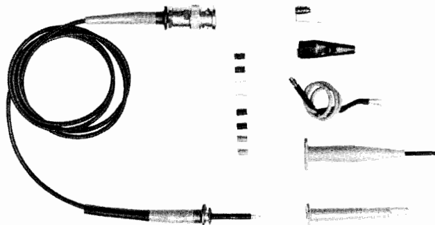
HP Models 10026A, 10027A
