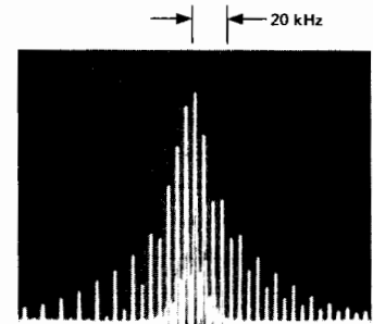
Spectrum Analyzer display of simultaneous AM (46.5%) and FM (4.5 kHz peak deviation) modulation.
