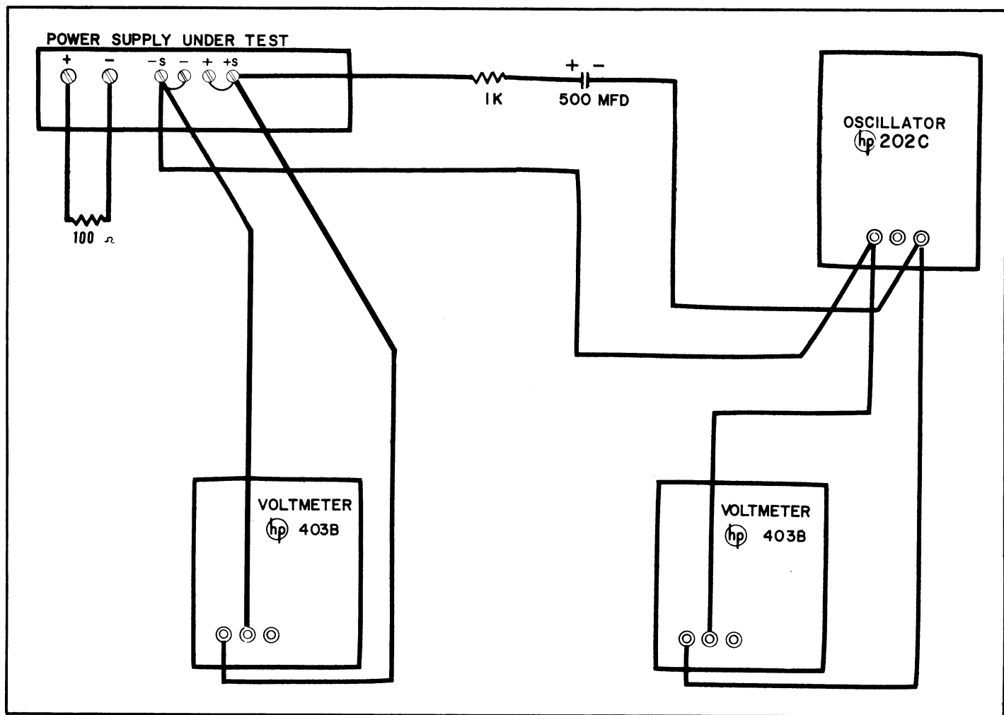
Figure 5-6. Output Impedance, Test Setup
