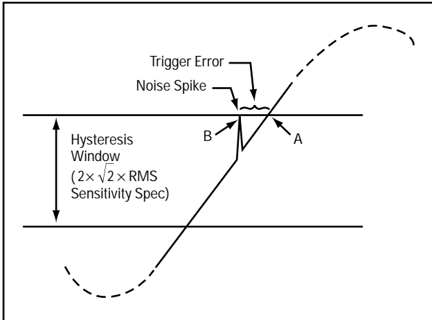
Figure 10. Trigger error.
