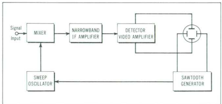
Fig. 3. Simplified block diagram of wide-band spectrum analyzer.
