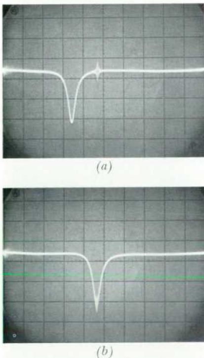
Fig. 3. Oscillograms showing dip produced by hp-537A Frequency Meter. Marker (derived from house frequency standard) is at 8.4 GHz. Cavity Q of Model 537A, measured on these oscillograms, is greater than 2000. (a) Wavemeter not tuned exactly to 8.4 GHz. (b) Wavemeter tuned to 8.4 GHz. Horizontal: 10 MHz/cm; Vertical: linear in power.
