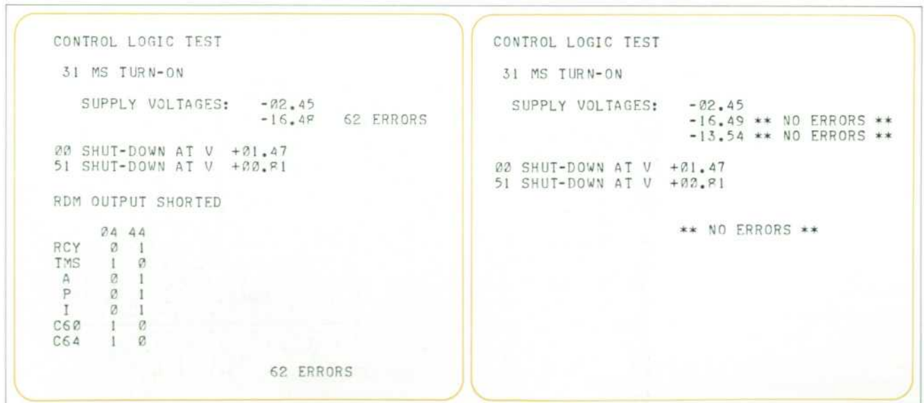
Fig. 3. Typical teleprinter output for a defective assembly (left), and printout for a perfect board (right).
